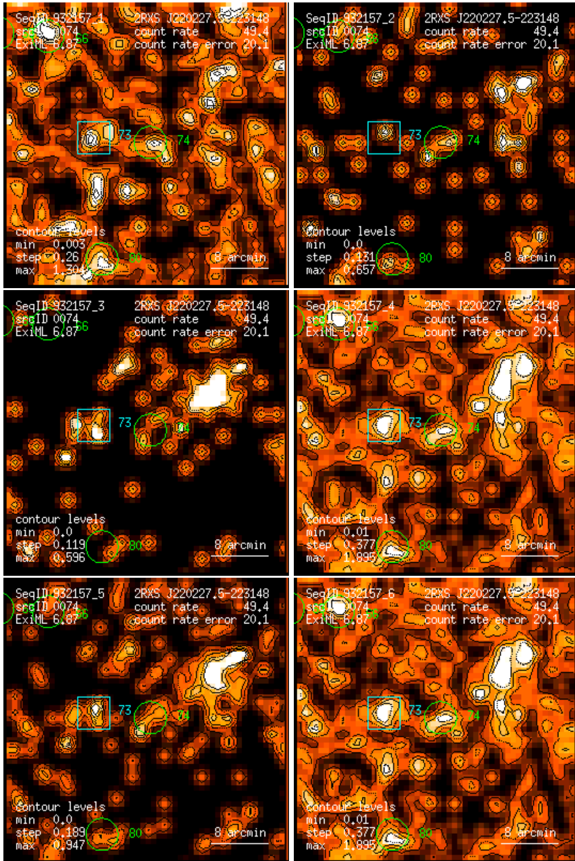
Figure 74: RASS 932157: detection 0074: band rate images, Gaussian filter: (1) PSPC channels 11 – 41, (2) 52 – 90, (3) 91 – 201, (4) 11 – 235, (5) 52 – 201, (6) 11 – 201. Broad band rates in counts/ks. Band rate contour levels in counts/ks/arcmin 2 .
