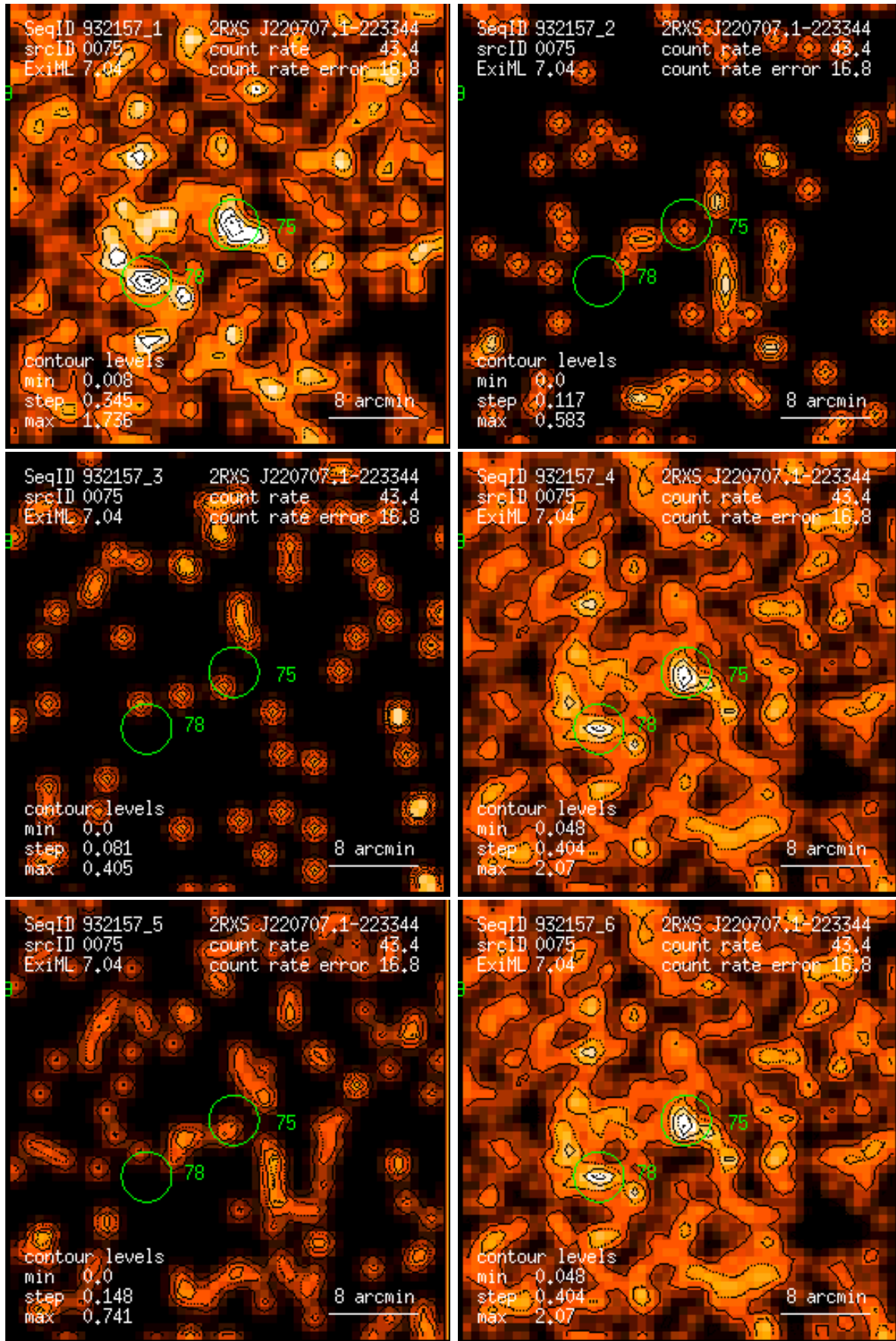
Figure 75: RASS 932157: detection 0075: band rate images, Gaussian filter: (1) PSPC channels 11 – 41, (2) 52 – 90, (3) 91 – 201, (4) 11 – 235, (5) 52 – 201, (6) 11 – 201. Broad band rates in counts/ks. Band rate contour levels in counts/ks/arcmin 2 .
