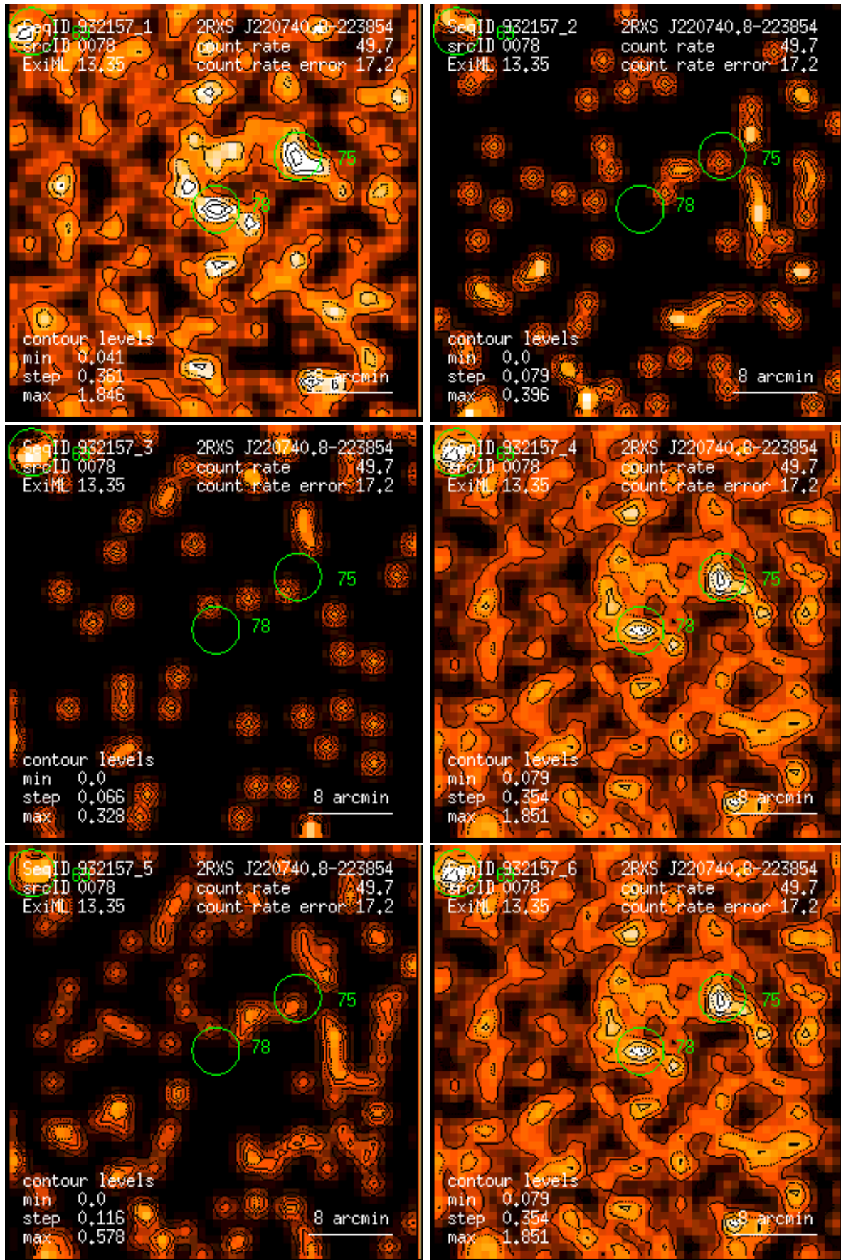
Figure 78: RASS 932157: detection 0078: band rate images, Gaussian filter: (1) PSPC channels 11 – 41, (2) 52 – 90, (3) 91 – 201, (4) 11 – 235, (5) 52 – 201, (6) 11 – 201. Broad band rates in counts/ks. Band rate contour levels in counts/ks/arcmin 2 .
