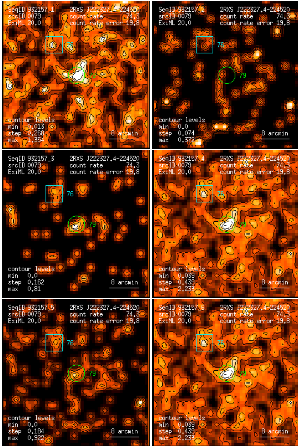
Figure 79: RASS 932157: detection 0079: band rate images, Gaussian filter: (1) PSPC channels 11 – 41, (2) 52 – 90, (3) 91 – 201, (4) 11 – 235, (5) 52 – 201, (6) 11 – 201. Broad band rates in counts/ks. Band rate contour levels in counts/ks/arcmin 2 .
