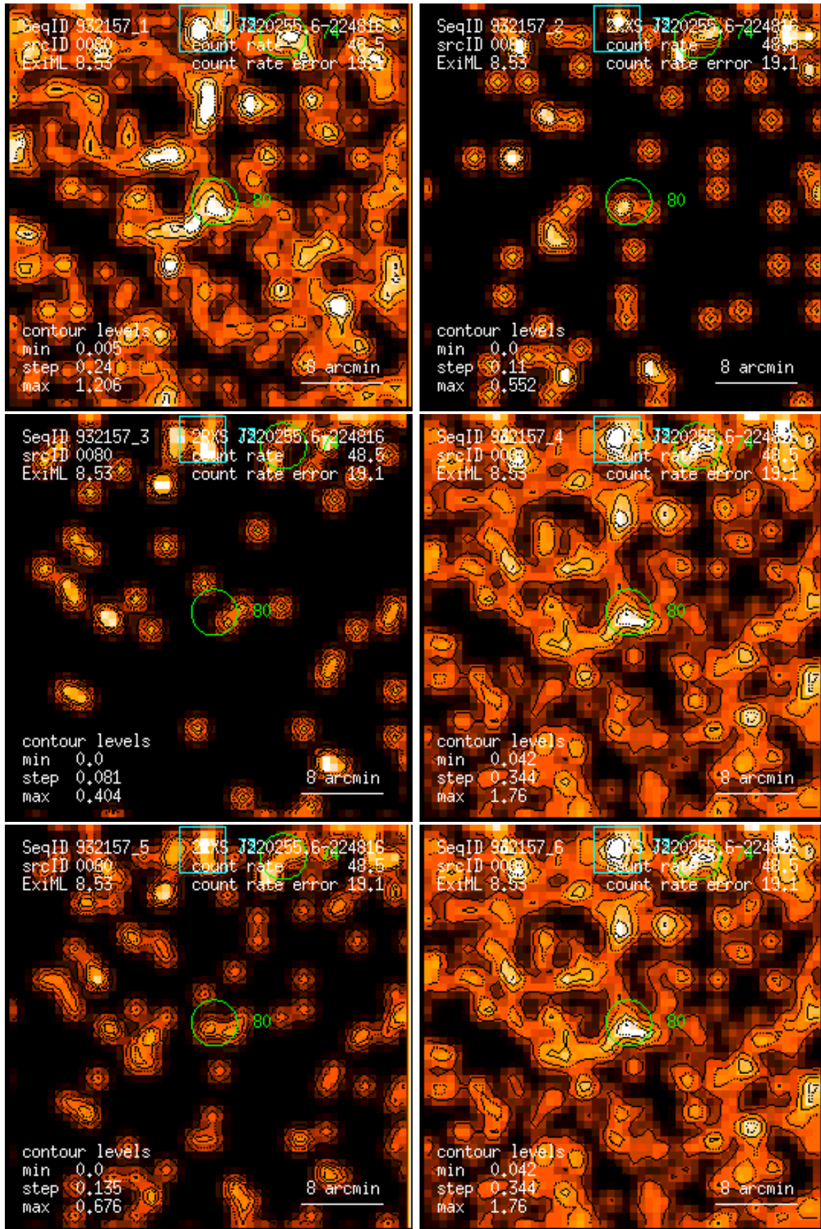
Figure 80: RASS 932157: detection 0080: band rate images, Gaussian filter: (1) PSPC channels 11 – 41, (2) 52 – 90, (3) 91 – 201, (4) 11 – 235, (5) 52 – 201, (6) 11 – 201. Broad band rates in counts/ks. Band rate contour levels in counts/ks/arcmin 2 .
