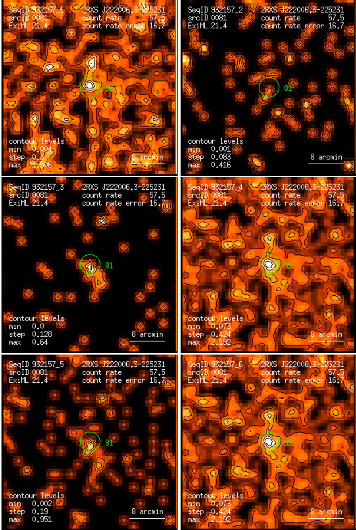
Figure 81: RASS 932157: detection 0081: band rate images, Gaussian filter: (1) PSPC channels 11 – 41, (2) 52 – 90, (3) 91 – 201, (4) 11 – 235, (5) 52 – 201, (6) 11 – 201. Broad band rates in counts/ks. Band rate contour levels in counts/ks/arcmin 2 .
