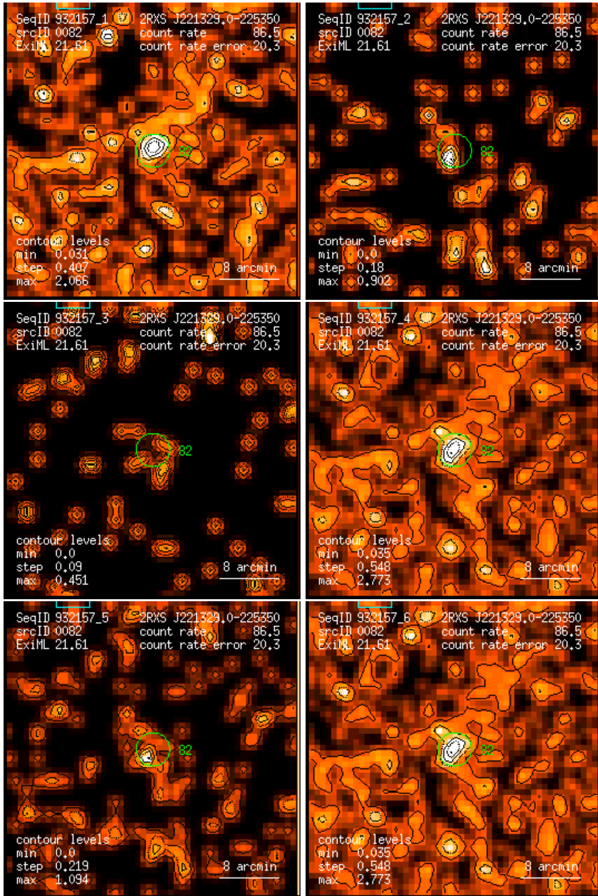
Figure 82: RASS 932157: detection 0082: band rate images, Gaussian filter: (1) PSPC channels 11 – 41, (2) 52 – 90, (3) 91 – 201, (4) 11 – 235, (5) 52 – 201, (6) 11 – 201. Broad band rates in counts/ks. Band rate contour levels in counts/ks/arcmin 2 .
