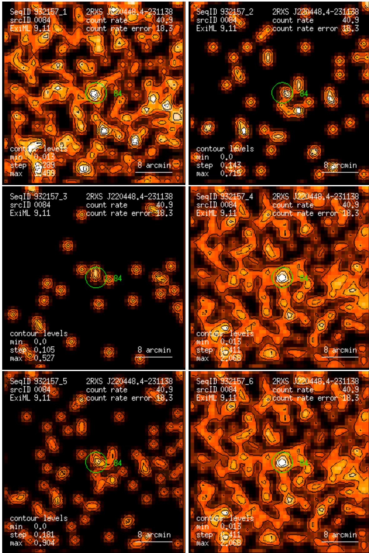
Figure 84: RASS 932157: detection 0084: band rate images, Gaussian filter: (1) PSPC channels 11 – 41, (2) 52 – 90, (3) 91 – 201, (4) 11 – 235, (5) 52 – 201, (6) 11 – 201. Broad band rates in counts/ks. Band rate contour levels in counts/ks/arcmin 2 .
