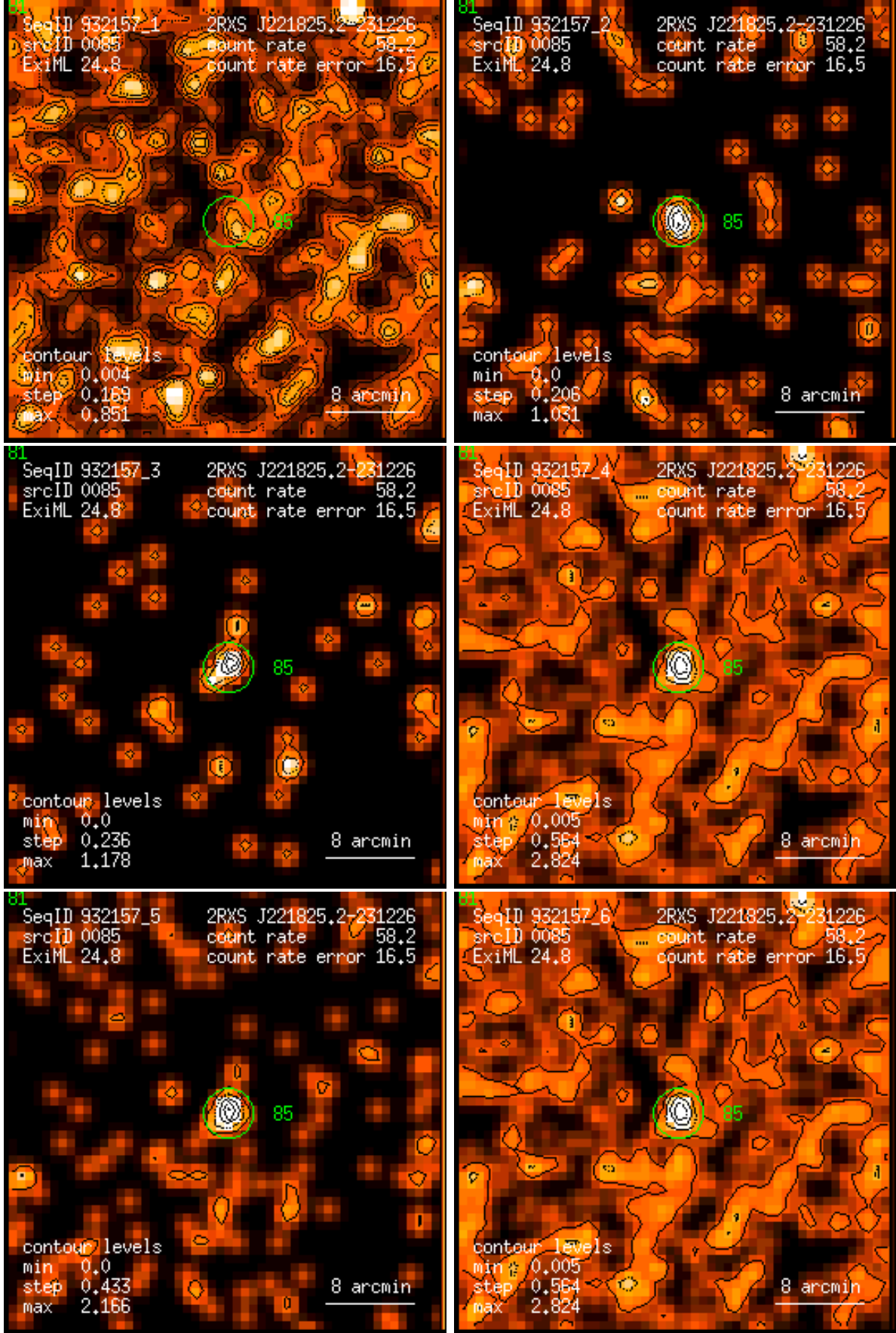
Figure 85: RASS 932157: detection 0085: band rate images, Gaussian filter: (1) PSPC channels 11 – 41, (2) 52 – 90, (3) 91 – 201, (4) 11 – 235, (5) 52 – 201, (6) 11 – 201. Broad band rates in counts/ks. Band rate contour levels in counts/ks/arcmin 2 .
