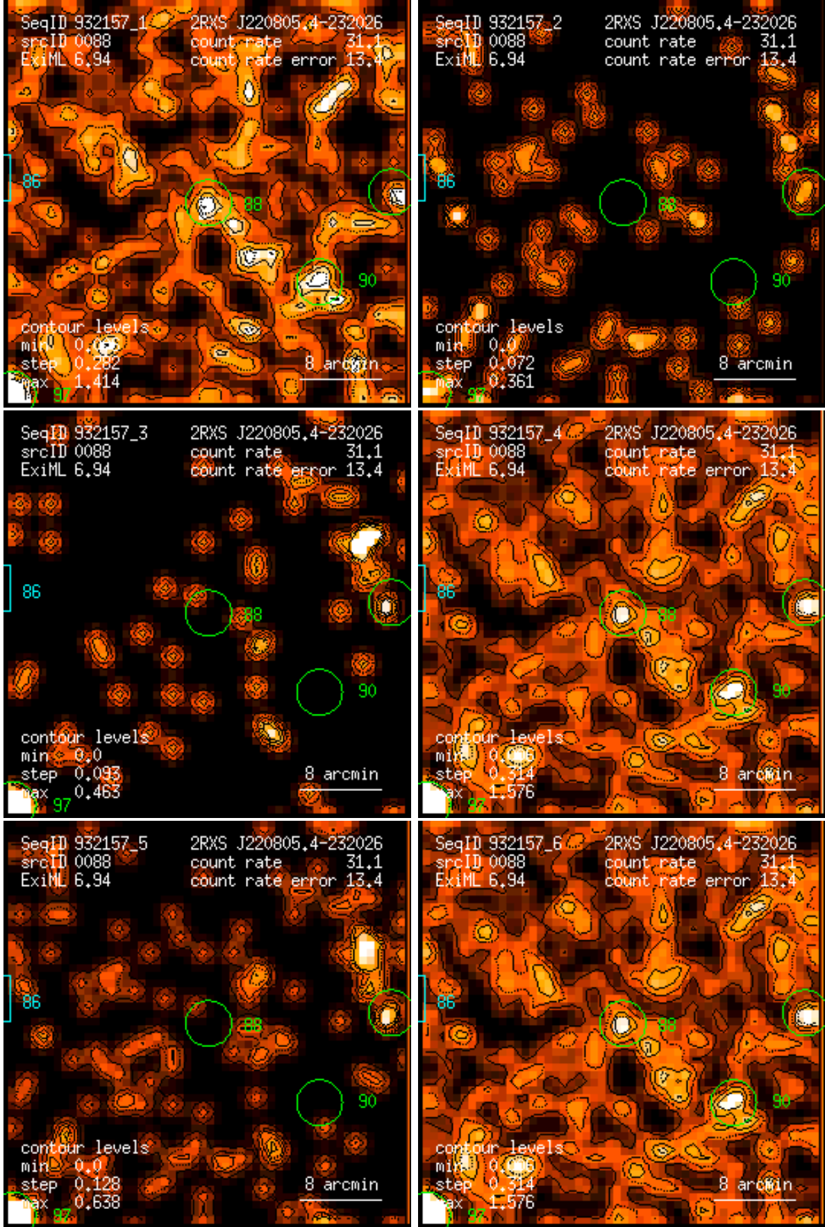
Figure 88: RASS 932157: detection 0088: band rate images, Gaussian filter: (1) PSPC channels 11 – 41, (2) 52 – 90, (3) 91 – 201, (4) 11 – 235, (5) 52 – 201, (6) 11 – 201. Broad band rates in counts/ks. Band rate contour levels in counts/ks/arcmin 2 .
