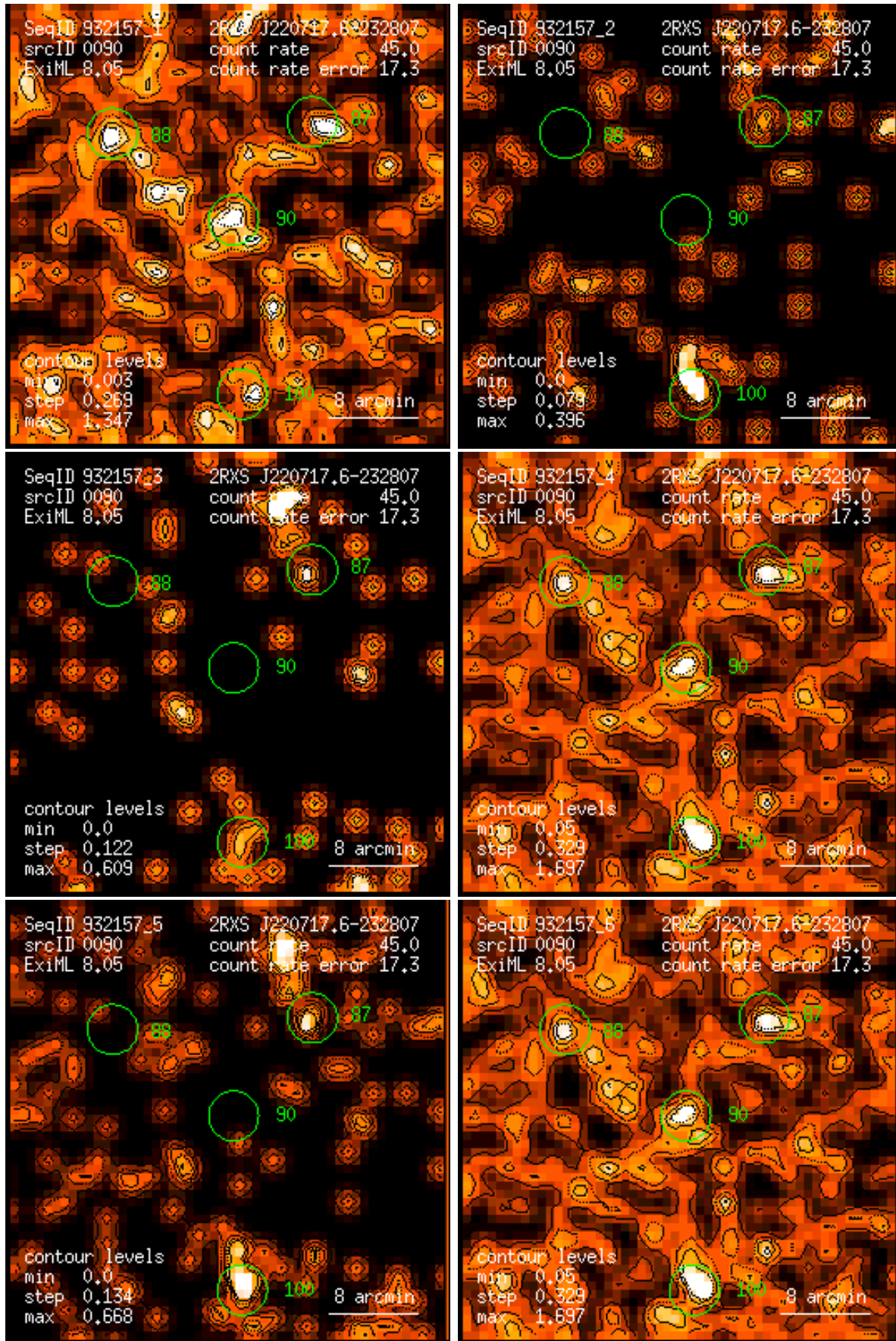
Figure 90: RASS 932157: detection 0090: band rate images, Gaussian filter: (1) PSPC channels 11 – 41, (2) 52 – 90, (3) 91 – 201, (4) 11 – 235, (5) 52 – 201, (6) 11 – 201. Broad band rates in counts/ks. Band rate contour levels in counts/ks/arcmin 2 .
