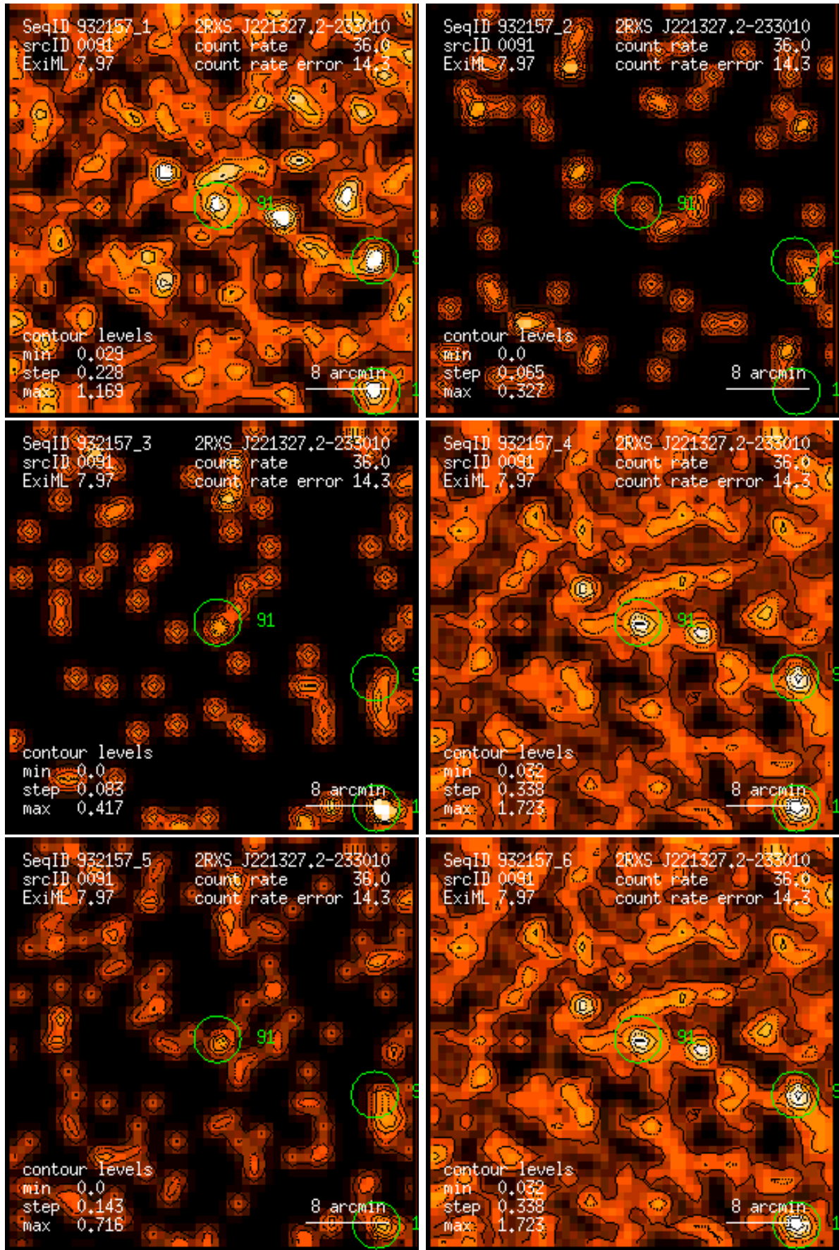
Figure 91: RASS 932157: detection 0091: band rate images, Gaussian filter: (1) PSPC channels 11 – 41, (2) 52 – 90, (3) 91 – 201, (4) 11 – 235, (5) 52 – 201, (6) 11 – 201. Broad band rates in counts/ks. Band rate contour levels in counts/ks/arcmin 2 .
