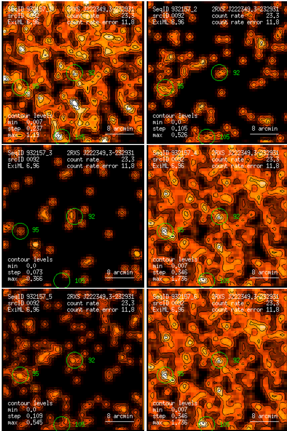
Figure 92: RASS 932157: detection 0092: band rate images, Gaussian filter: (1) PSPC channels 11 – 41, (2) 52 – 90, (3) 91 – 201, (4) 11 – 235, (5) 52 – 201, (6) 11 – 201. Broad band rates in counts/ks. Band rate contour levels in counts/ks/arcmin 2 .
