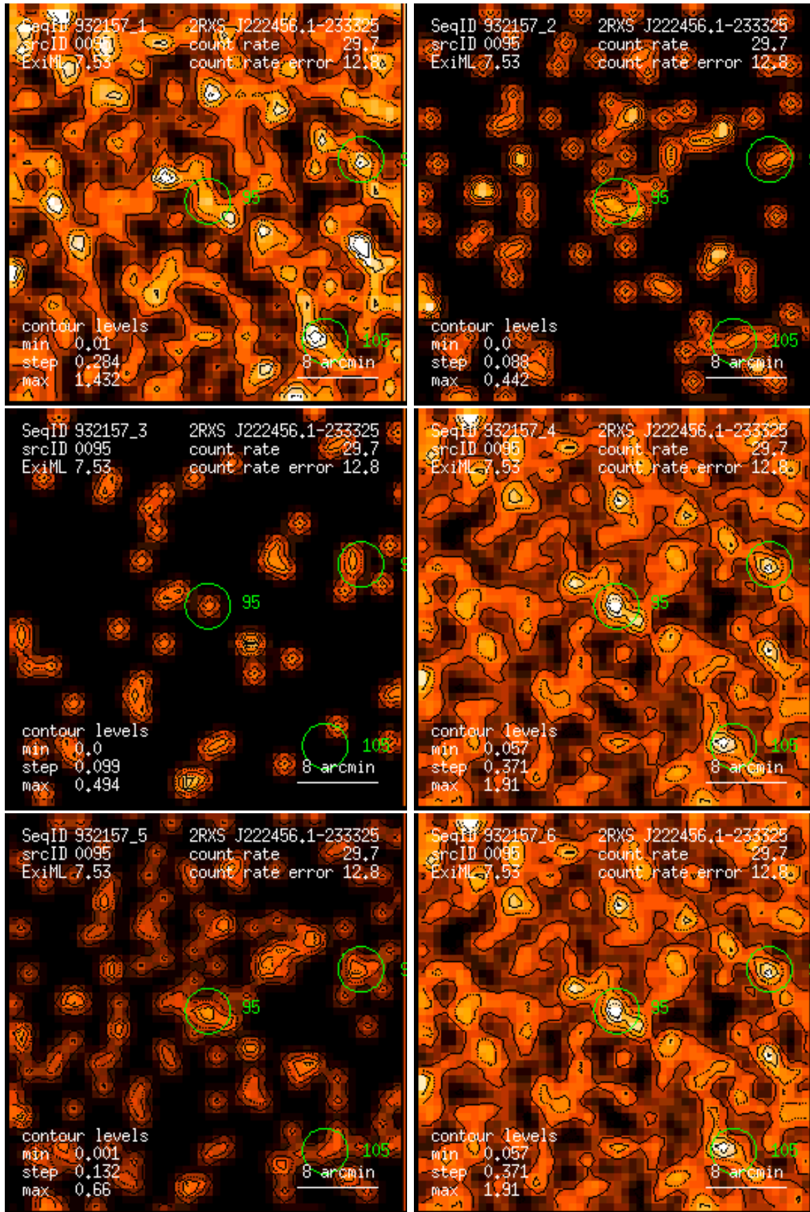
Figure 95: RASS 932157: detection 0095: band rate images, Gaussian filter: (1) PSPC channels 11 – 41, (2) 52 – 90, (3) 91 – 201, (4) 11 – 235, (5) 52 – 201, (6) 11 – 201. Broad band rates in counts/ks. Band rate contour levels in counts/ks/arcmin 2 .
