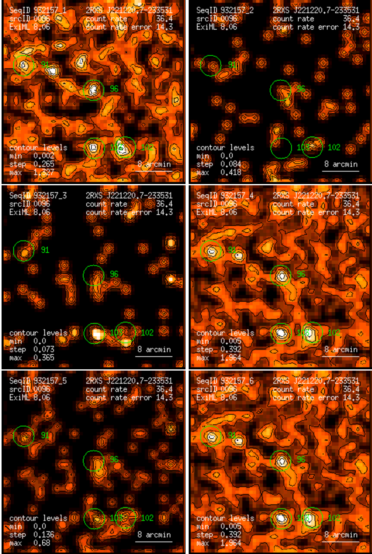
Figure 96: RASS 932157: detection 0096: band rate images, Gaussian filter: (1) PSPC channels 11 – 41, (2) 52 – 90, (3) 91 – 201, (4) 11 – 235, (5) 52 – 201, (6) 11 – 201. Broad band rates in counts/ks. Band rate contour levels in counts/ks/arcmin 2 .
