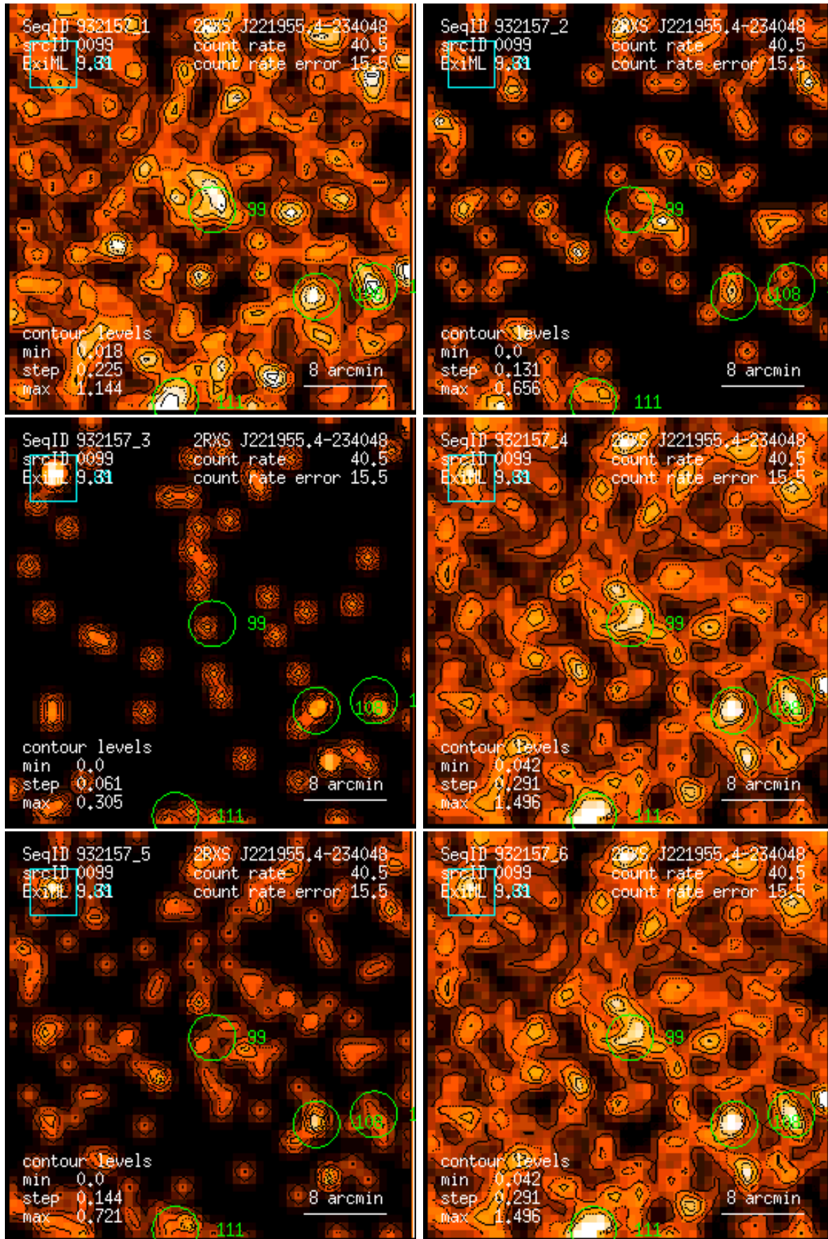
Figure 99: RASS 932157: detection 0099: band rate images, Gaussian filter: (1) PSPC channels 11 – 41, (2) 52 – 90, (3) 91 – 201, (4) 11 – 235, (5) 52 – 201, (6) 11 – 201. Broad band rates in counts/ks. Band rate contour levels in counts/ks/arcmin 2 .
