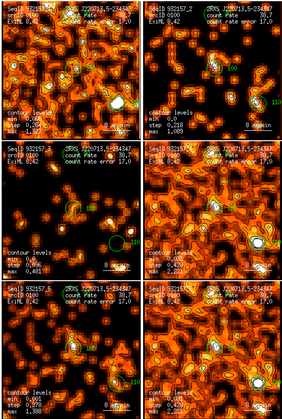
Figure 100: RASS 932157: detection 0100: band rate images, Gaussian filter: (1) PSPC channels 11 – 41, (2) 52 – 90, (3) 91 – 201, (4) 11 – 235, (5) 52 – 201, (6) 11 – 201. Broad band rates in counts/ks. Band rate contour levels in counts/ks/arcmin 2 .
