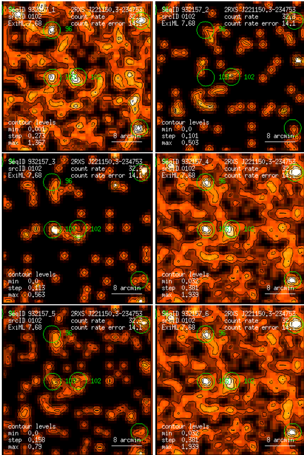
Figure 102: RASS 932157: detection 0102: band rate images, Gaussian filter: (1) PSPC channels 11 – 41, (2) 52 – 90, (3) 91 – 201, (4) 11 – 235, (5) 52 – 201, (6) 11 – 201. Broad band rates in counts/ks. Band rate contour levels in counts/ks/arcmin 2 .
