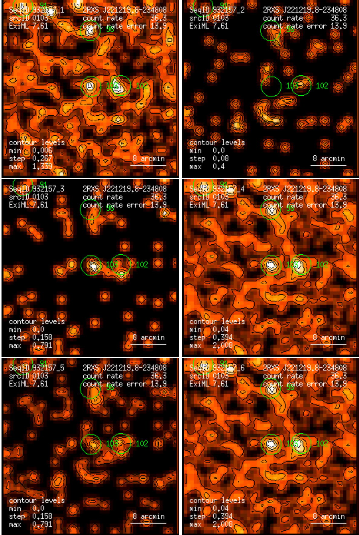
Figure 103: RASS 932157: detection 0103: band rate images, Gaussian filter: (1) PSPC channels 11 – 41, (2) 52 – 90, (3) 91 – 201, (4) 11 – 235, (5) 52 – 201, (6) 11 – 201. Broad band rates in counts/ks. Band rate contour levels in counts/ks/arcmin 2 .
