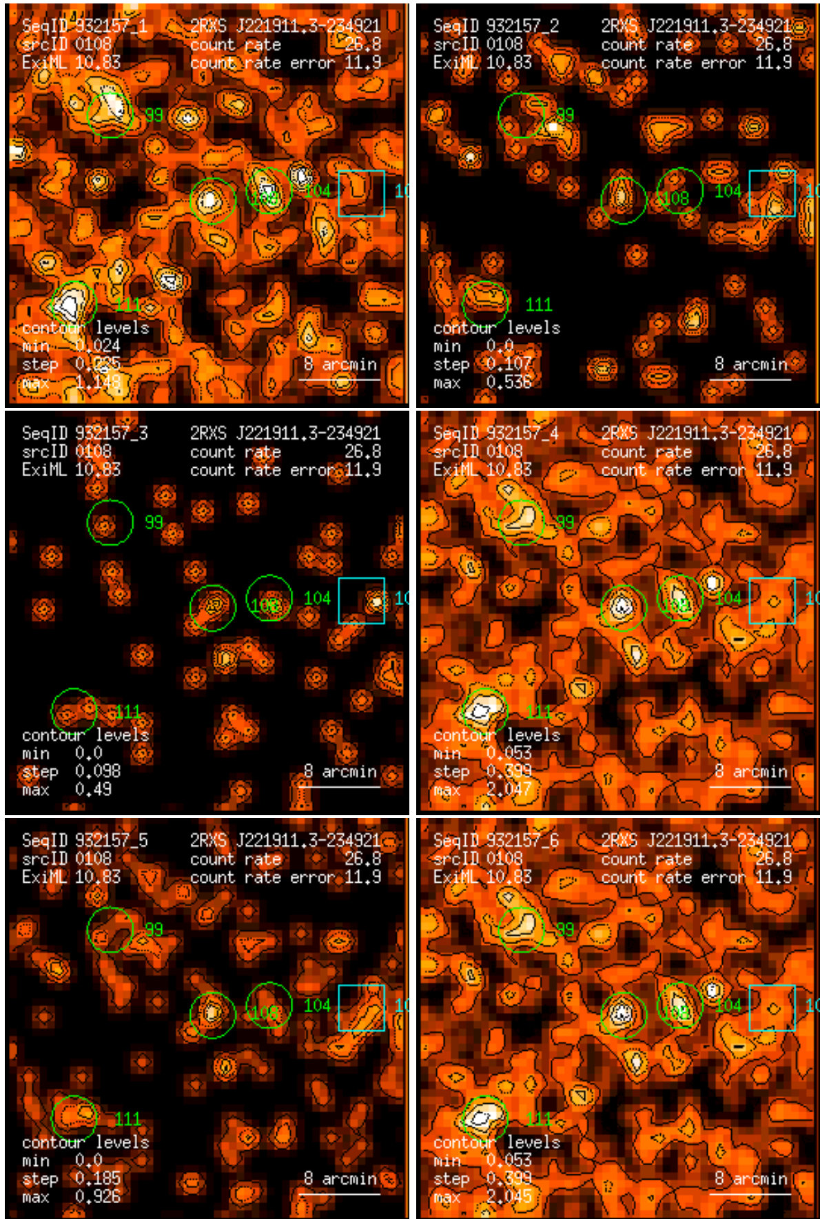
Figure 108: RASS 932157: detection 0108: band rate images, Gaussian filter: (1) PSPC channels 11 – 41, (2) 52 – 90, (3) 91 – 201, (4) 11 – 235, (5) 52 – 201, (6) 11 – 201. Broad band rates in counts/ks. Band rate contour levels in counts/ks/arcmin 2 .
