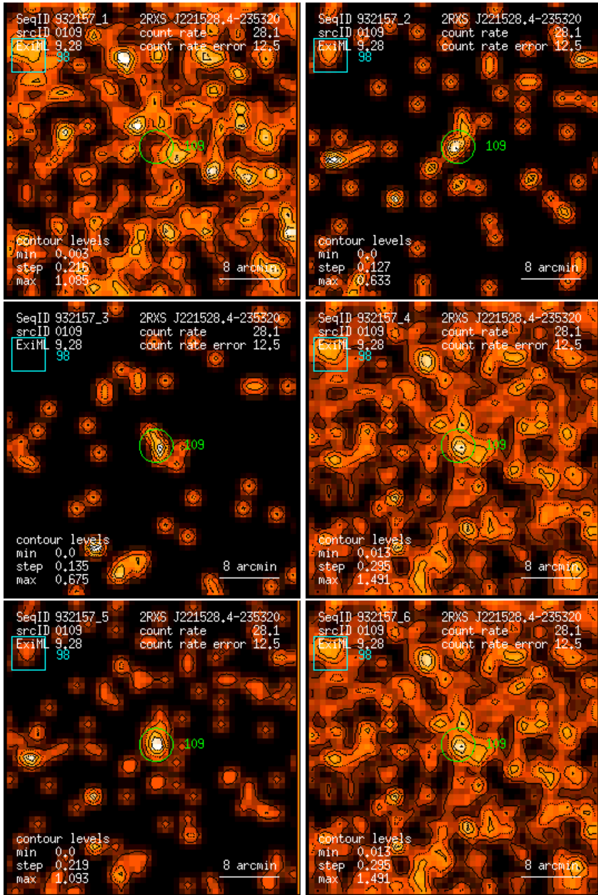
Figure 109: RASS 932157: detection 0109: band rate images, Gaussian filter: (1) PSPC channels 11 – 41, (2) 52 – 90, (3) 91 – 201, (4) 11 – 235, (5) 52 – 201, (6) 11 – 201. Broad band rates in counts/ks. Band rate contour levels in counts/ks/arcmin 2 .
