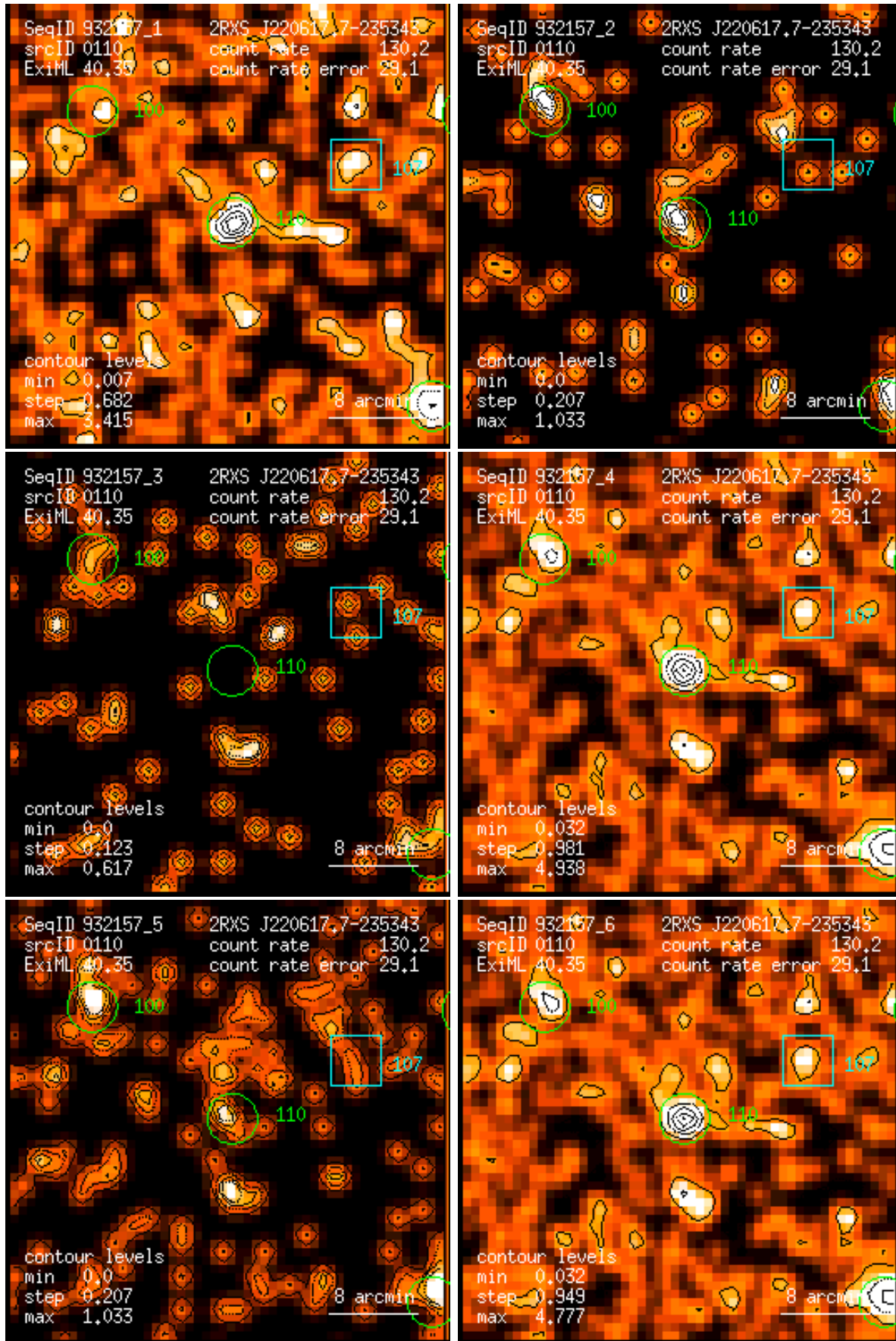
Figure 110: RASS 932157: detection 0110: band rate images, Gaussian filter: (1) PSPC channels 11 – 41, (2) 52 – 90, (3) 91 – 201, (4) 11 – 235, (5) 52 – 201, (6) 11 – 201. Broad band rates in counts/ks. Band rate contour levels in counts/ks/arcmin 2 .
