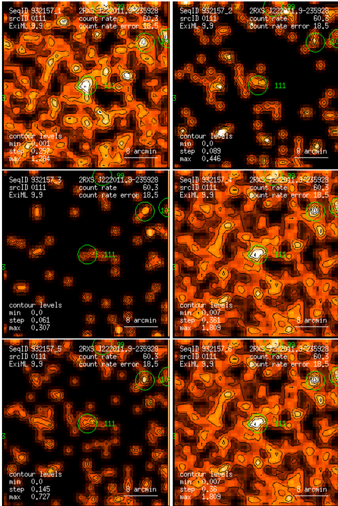
Figure 111: RASS 932157: detection 0111: band rate images, Gaussian filter: (1) PSPC channels 11 – 41, (2) 52 – 90, (3) 91 – 201, (4) 11 – 235, (5) 52 – 201, (6) 11 – 201. Broad band rates in counts/ks. Band rate contour levels in counts/ks/arcmin 2 .
