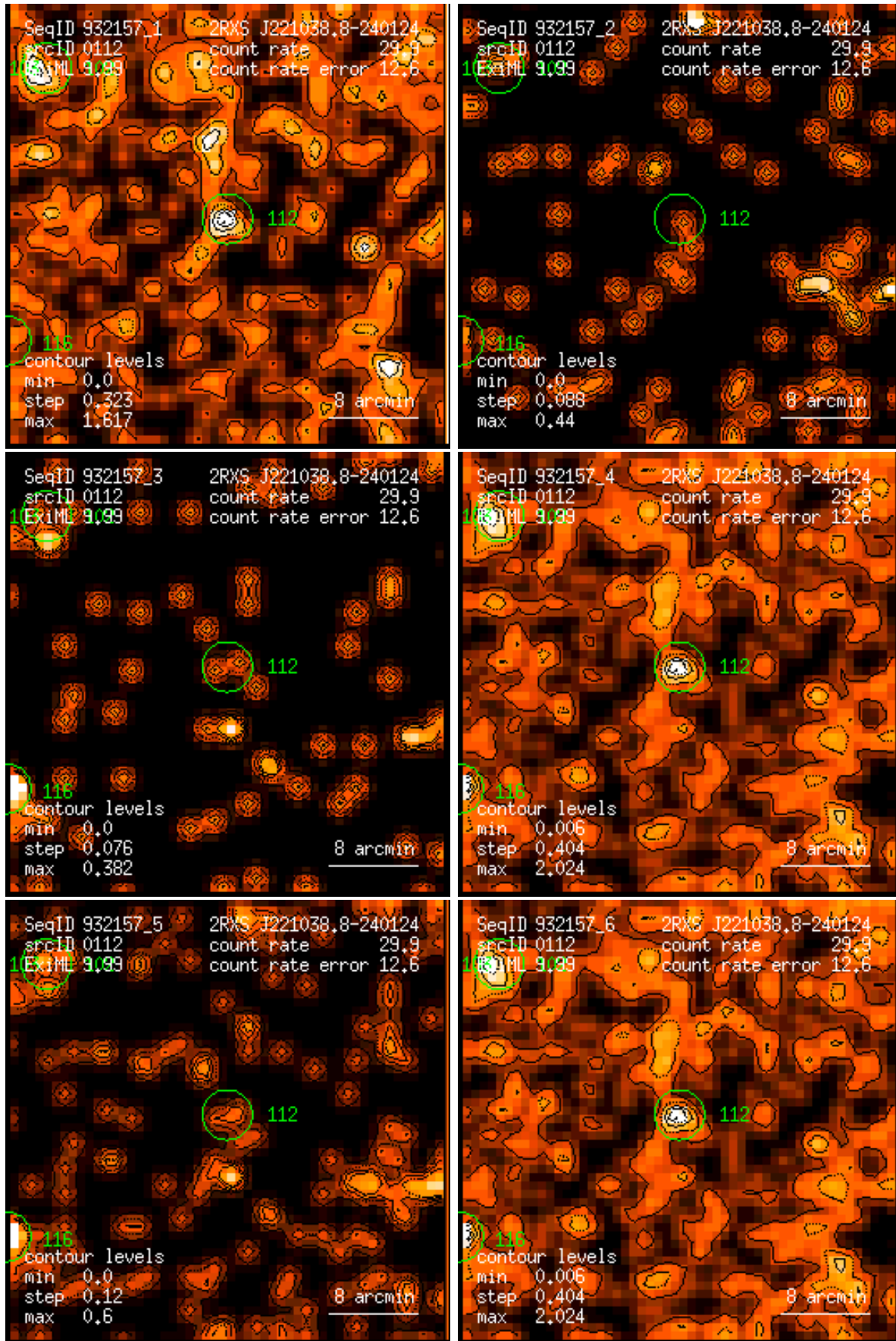
Figure 112: RASS 932157: detection 0112: band rate images, Gaussian filter: (1) PSPC channels 11 – 41, (2) 52 – 90, (3) 91 – 201, (4) 11 – 235, (5) 52 – 201, (6) 11 – 201. Broad band rates in counts/ks. Band rate contour levels in counts/ks/arcmin 2 .
