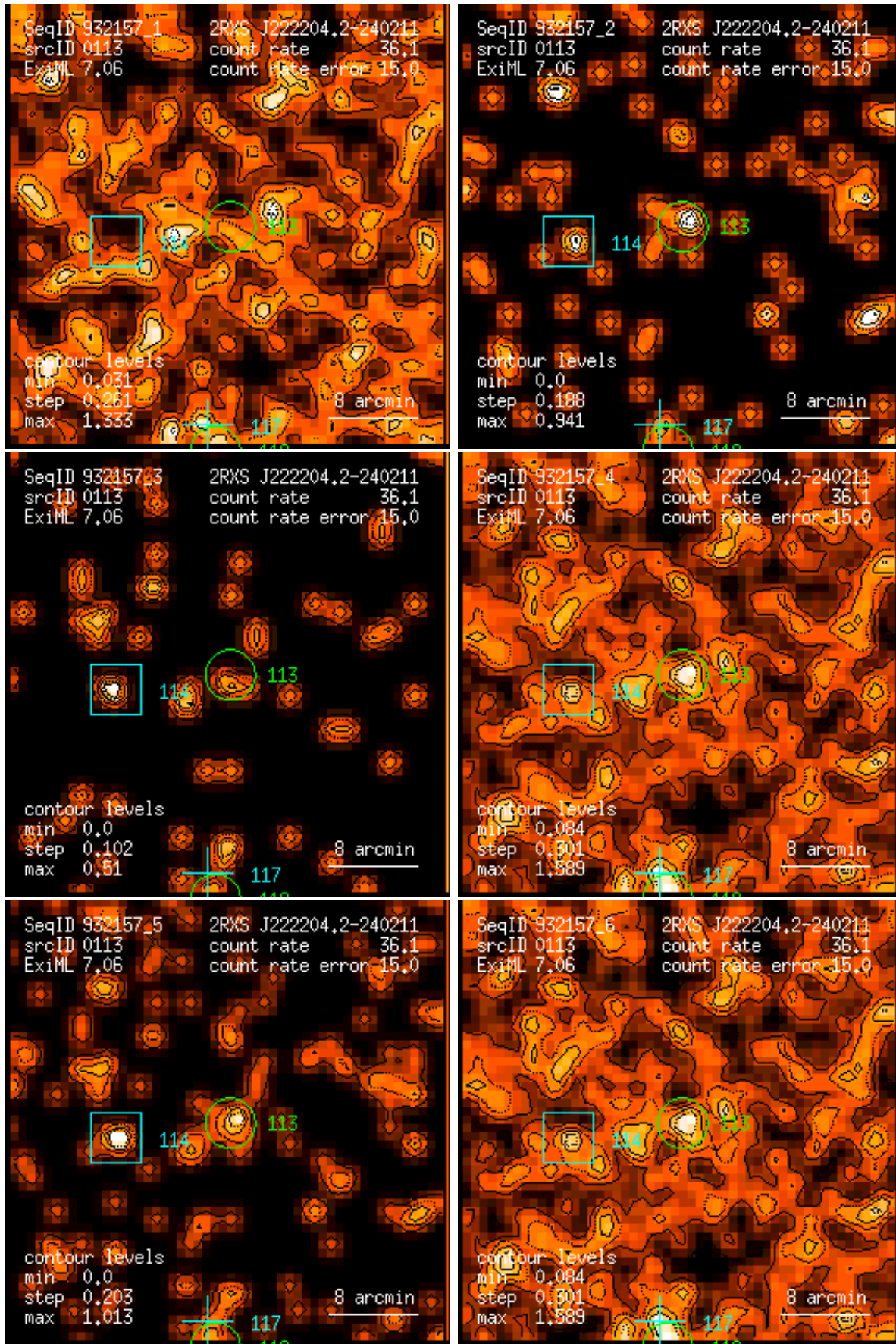
Figure 113: RASS 932157: detection 0113: band rate images, Gaussian filter: (1) PSPC channels 11 – 41, (2) 52 – 90, (3) 91 – 201, (4) 11 – 235, (5) 52 – 201, (6) 11 – 201. Broad band rates in counts/ks. Band rate contour levels in counts/ks/arcmin 2 .
