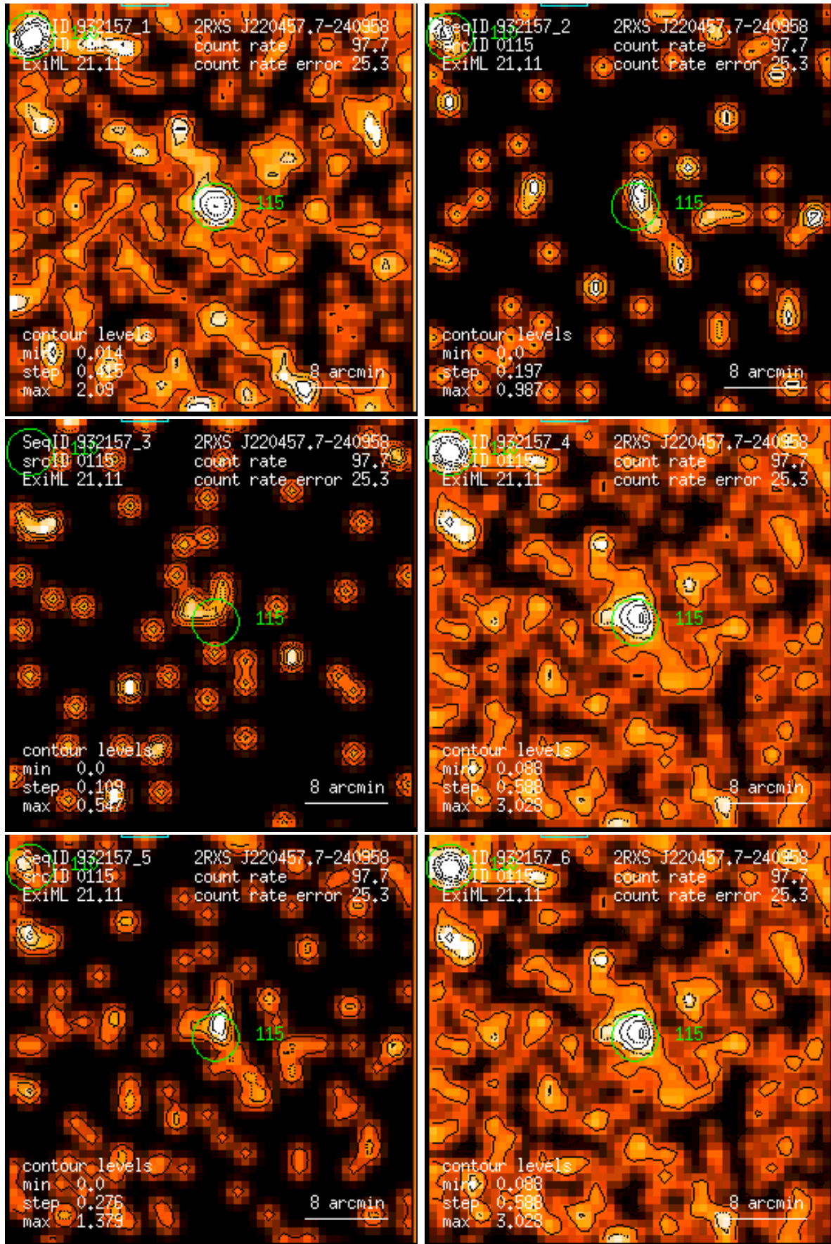
Figure 115: RASS 932157: detection 0115: band rate images, Gaussian filter: (1) PSPC channels 11 – 41, (2) 52 – 90, (3) 91 – 201, (4) 11 – 235, (5) 52 – 201, (6) 11 – 201. Broad band rates in counts/ks. Band rate contour levels in counts/ks/arcmin 2 .
