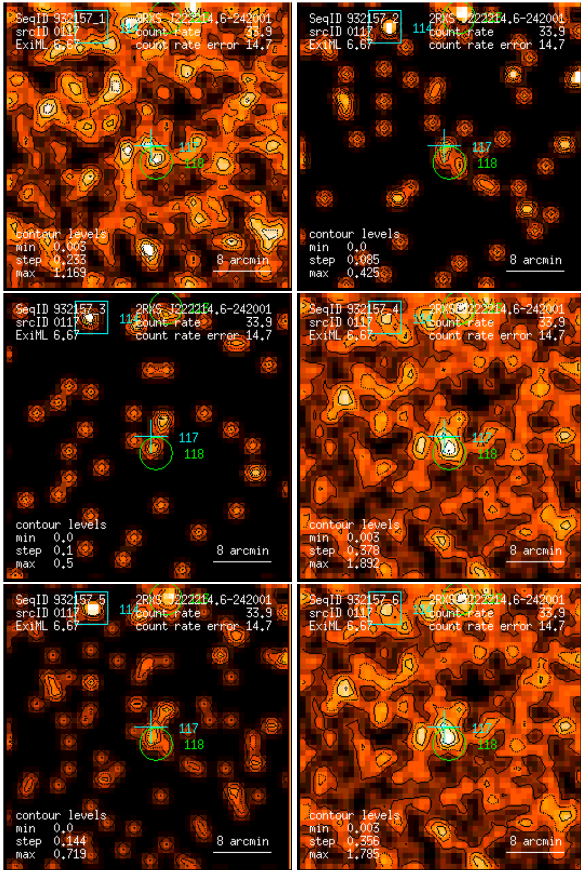
Figure 117: RASS 932157: detection 0117: band rate images, Gaussian filter: (1) PSPC channels 11 – 41, (2) 52 – 90, (3) 91 – 201, (4) 11 – 235, (5) 52 – 201, (6) 11 – 201. Broad band rates in counts/ks. Band rate contour levels in counts/ks/arcmin 2 .
