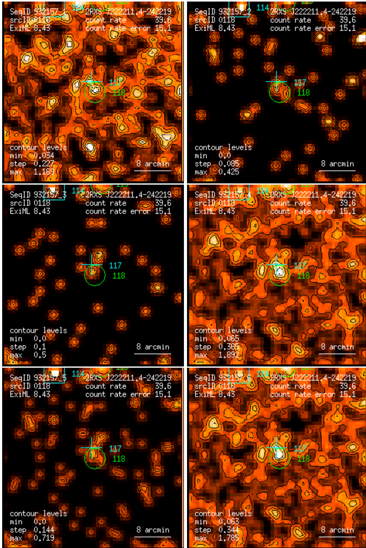
Figure 118: RASS 932157: detection 0118: band rate images, Gaussian filter: (1) PSPC channels 11 – 41, (2) 52 – 90, (3) 91 – 201, (4) 11 – 235, (5) 52 – 201, (6) 11 – 201. Broad band rates in counts/ks. Band rate contour levels in counts/ks/arcmin 2 .
