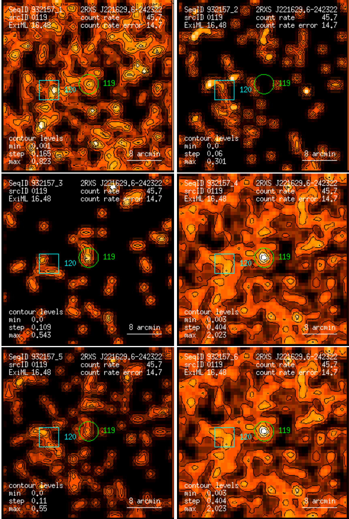
Figure 119: RASS 932157: detection 0119: band rate images, Gaussian filter: (1) PSPC channels 11 – 41, (2) 52 – 90, (3) 91 – 201, (4) 11 – 235, (5) 52 – 201, (6) 11 – 201. Broad band rates in counts/ks. Band rate contour levels in counts/ks/arcmin 2 .
