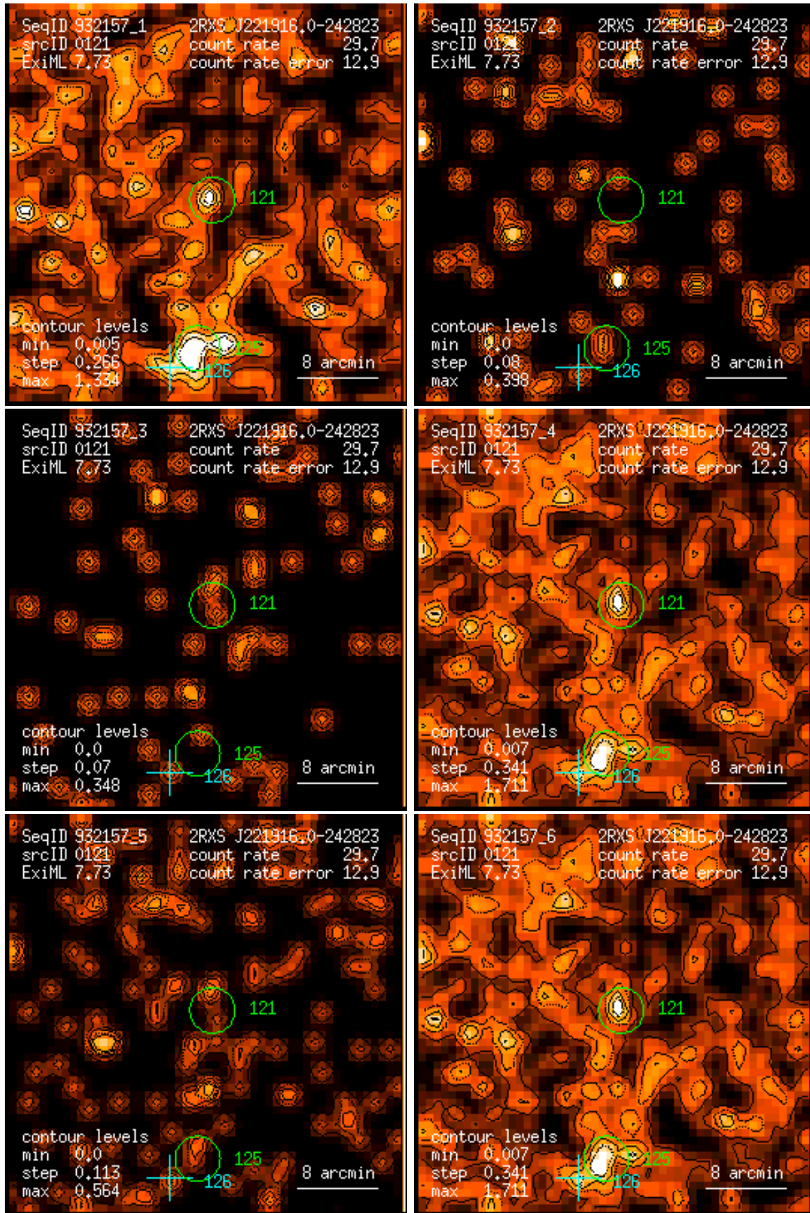
Figure 121: RASS 932157: detection 0121: band rate images, Gaussian filter: (1) PSPC channels 11 – 41, (2) 52 – 90, (3) 91 – 201, (4) 11 – 235, (5) 52 – 201, (6) 11 – 201. Broad band rates in counts/ks. Band rate contour levels in counts/ks/arcmin 2 .
