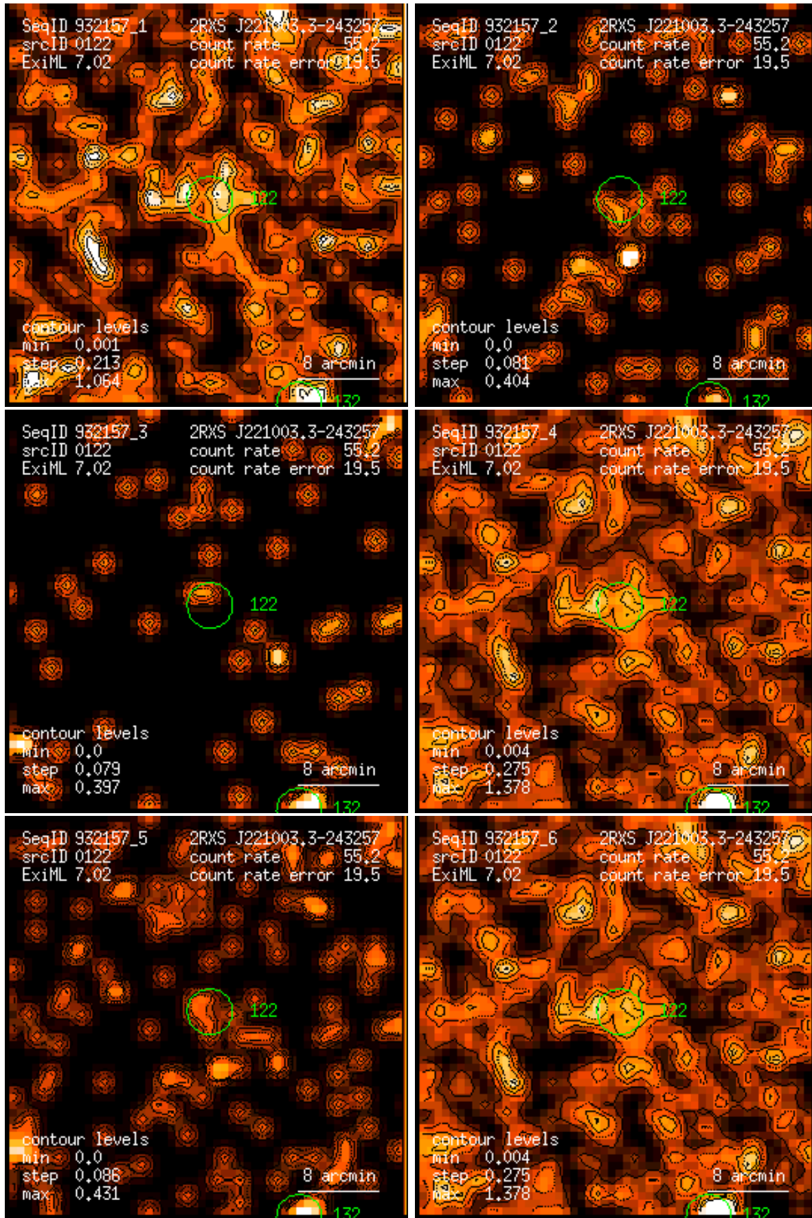
Figure 122: RASS 932157: detection 0122: band rate images, Gaussian filter: (1) PSPC channels 11 – 41, (2) 52 – 90, (3) 91 – 201, (4) 11 – 235, (5) 52 – 201, (6) 11 – 201. Broad band rates in counts/ks. Band rate contour levels in counts/ks/arcmin 2 .
