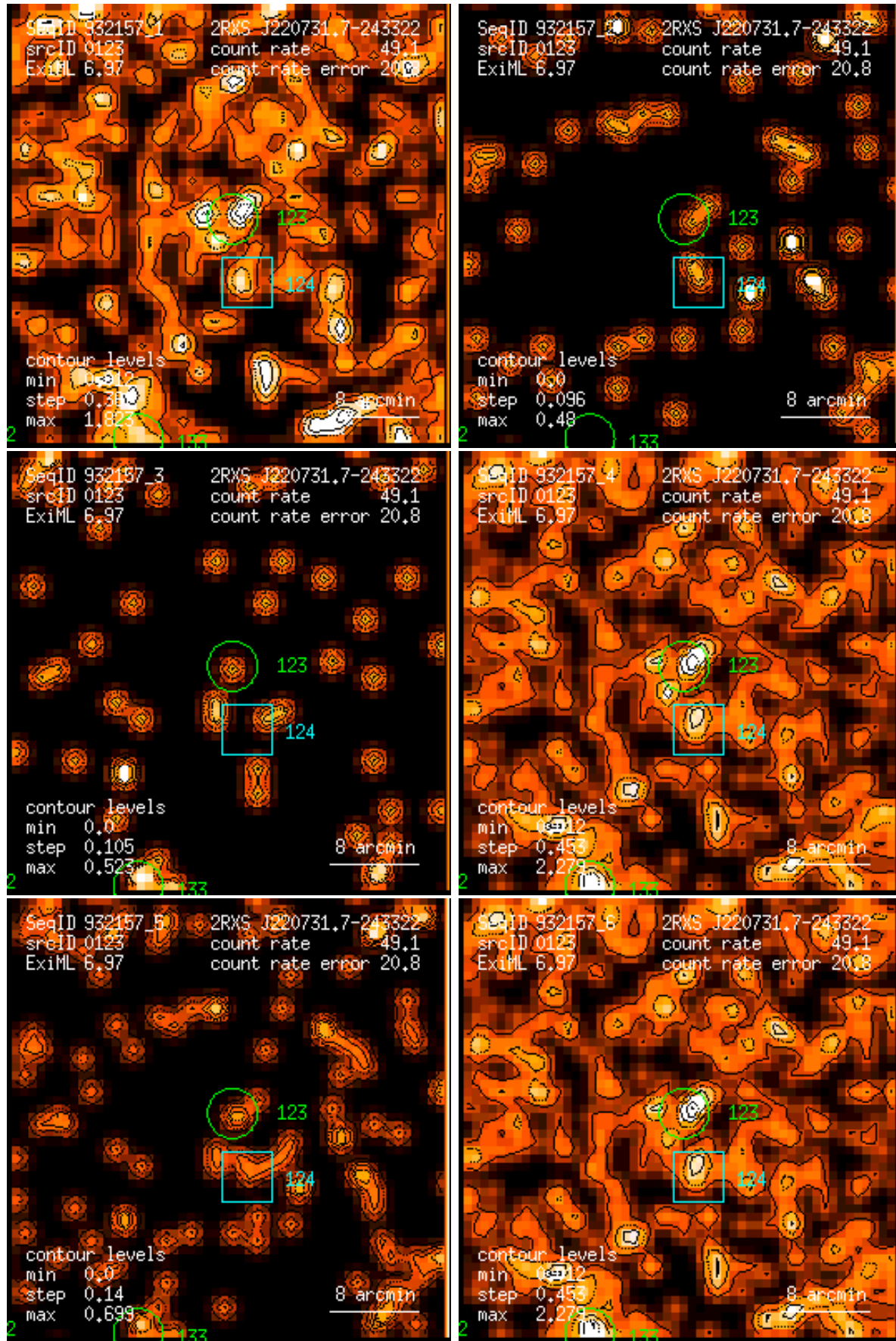
Figure 123: RASS 932157: detection 0123: band rate images, Gaussian filter: (1) PSPC channels 11 – 41, (2) 52 – 90, (3) 91 – 201, (4) 11 – 235, (5) 52 – 201, (6) 11 – 201. Broad band rates in counts/ks. Band rate contour levels in counts/ks/arcmin 2 .
