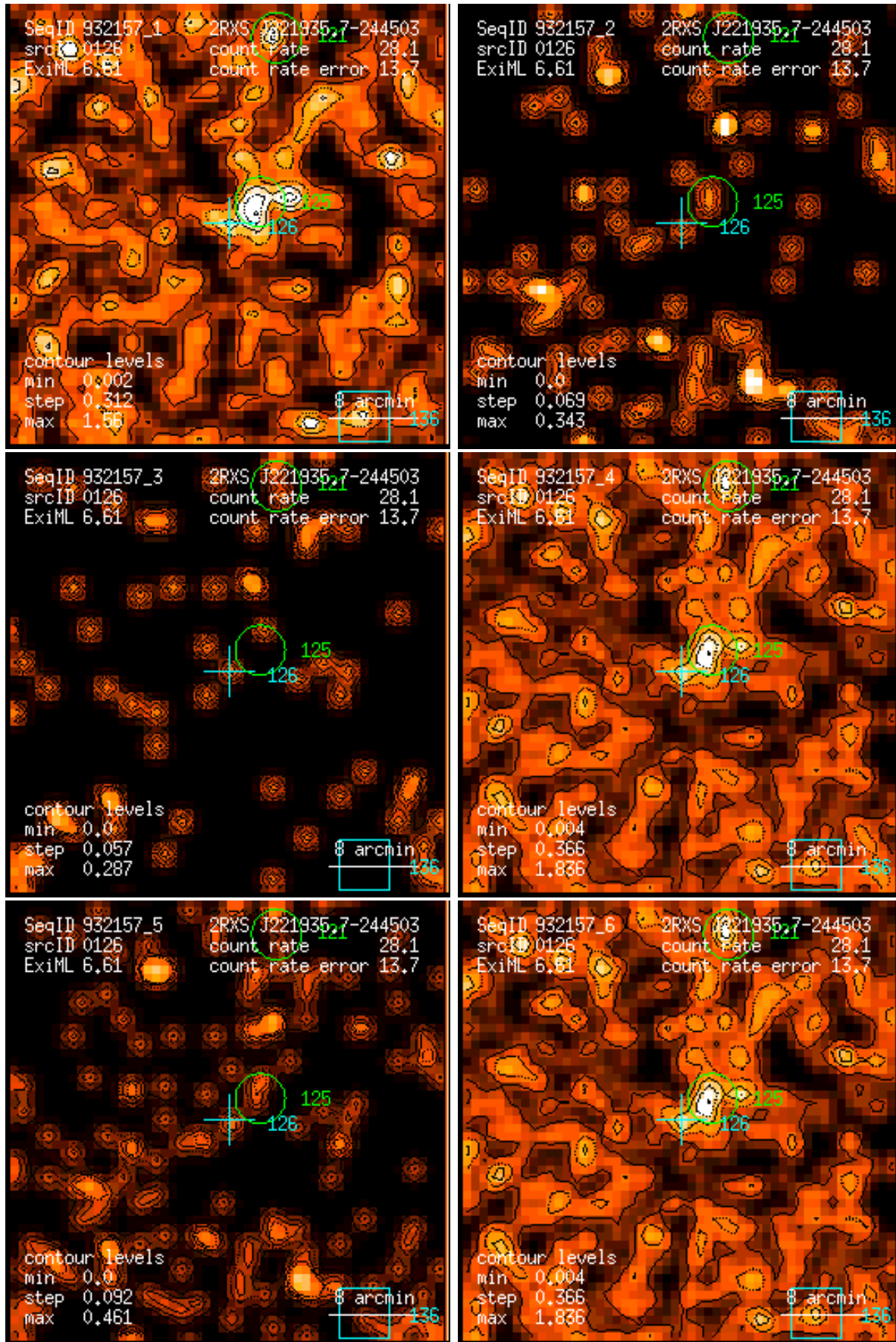
Figure 126: RASS 932157: detection 0126: band rate images, Gaussian filter: (1) PSPC channels 11 – 41, (2) 52 – 90, (3) 91 – 201, (4) 11 – 235, (5) 52 – 201, (6) 11 – 201. Broad band rates in counts/ks. Band rate contour levels in counts/ks/arcmin 2 .
