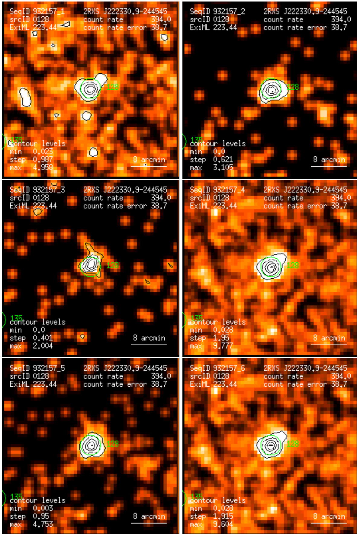
Figure 128: RASS 932157: detection 0128: band rate images, Gaussian filter: (1) PSPC channels 11 – 41, (2) 52 – 90, (3) 91 – 201, (4) 11 – 235, (5) 52 – 201, (6) 11 – 201. Broad band rates in counts/ks. Band rate contour levels in counts/ks/arcmin 2 .
