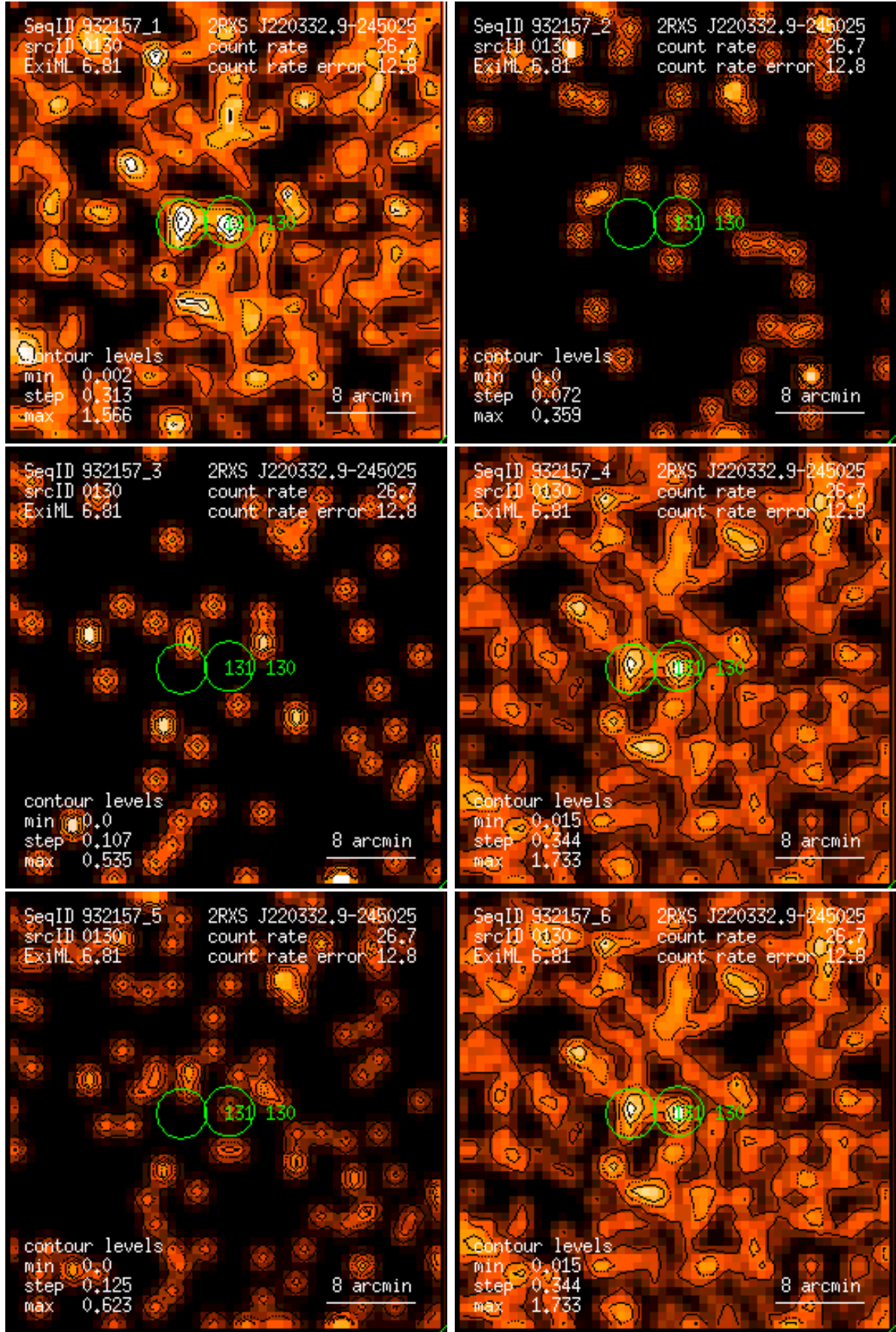
Figure 130: RASS 932157: detection 0130: band rate images, Gaussian filter: (1) PSPC channels 11 – 41, (2) 52 – 90, (3) 91 – 201, (4) 11 – 235, (5) 52 – 201, (6) 11 – 201. Broad band rates in counts/ks. Band rate contour levels in counts/ks/arcmin 2 .
