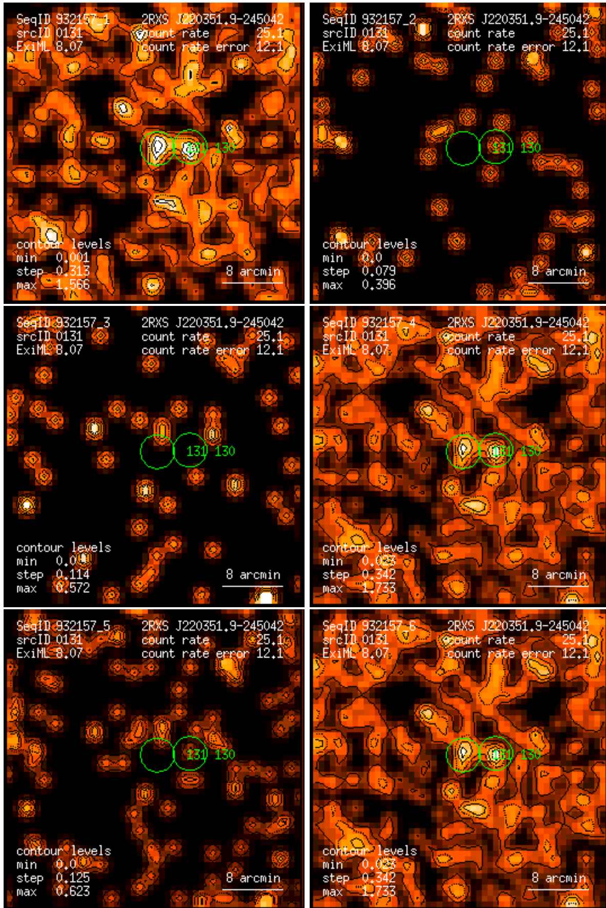
Figure 131: RASS 932157: detection 0131: band rate images, Gaussian filter: (1) PSPC channels 11 – 41, (2) 52 – 90, (3) 91 – 201, (4) 11 – 235, (5) 52 – 201, (6) 11 – 201. Broad band rates in counts/ks. Band rate contour levels in counts/ks/arcmin 2 .
