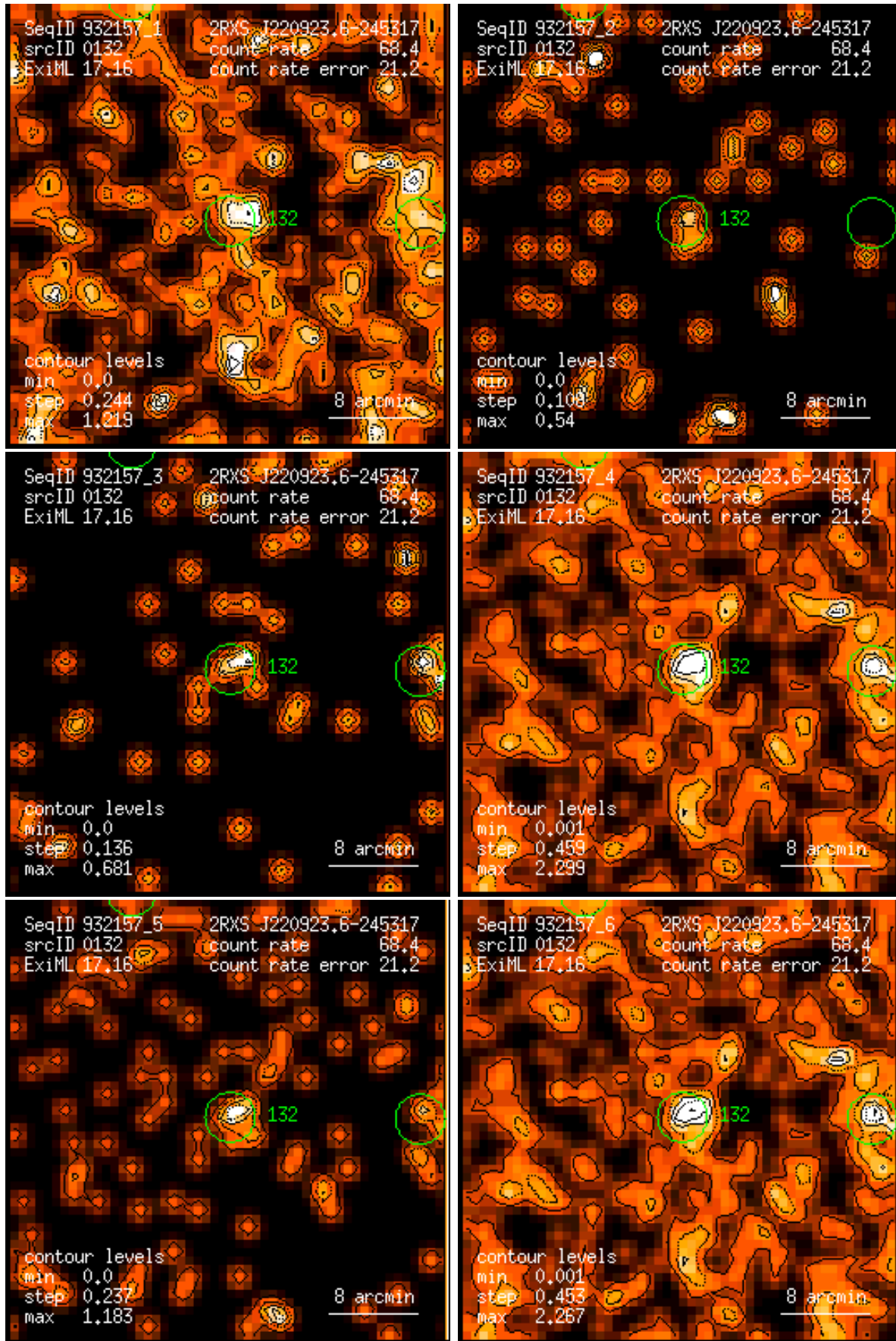
Figure 132: RASS 932157: detection 0132: band rate images, Gaussian filter: (1) PSPC channels 11 – 41, (2) 52 – 90, (3) 91 – 201, (4) 11 – 235, (5) 52 – 201, (6) 11 – 201. Broad band rates in counts/ks. Band rate contour levels in counts/ks/arcmin 2 .
