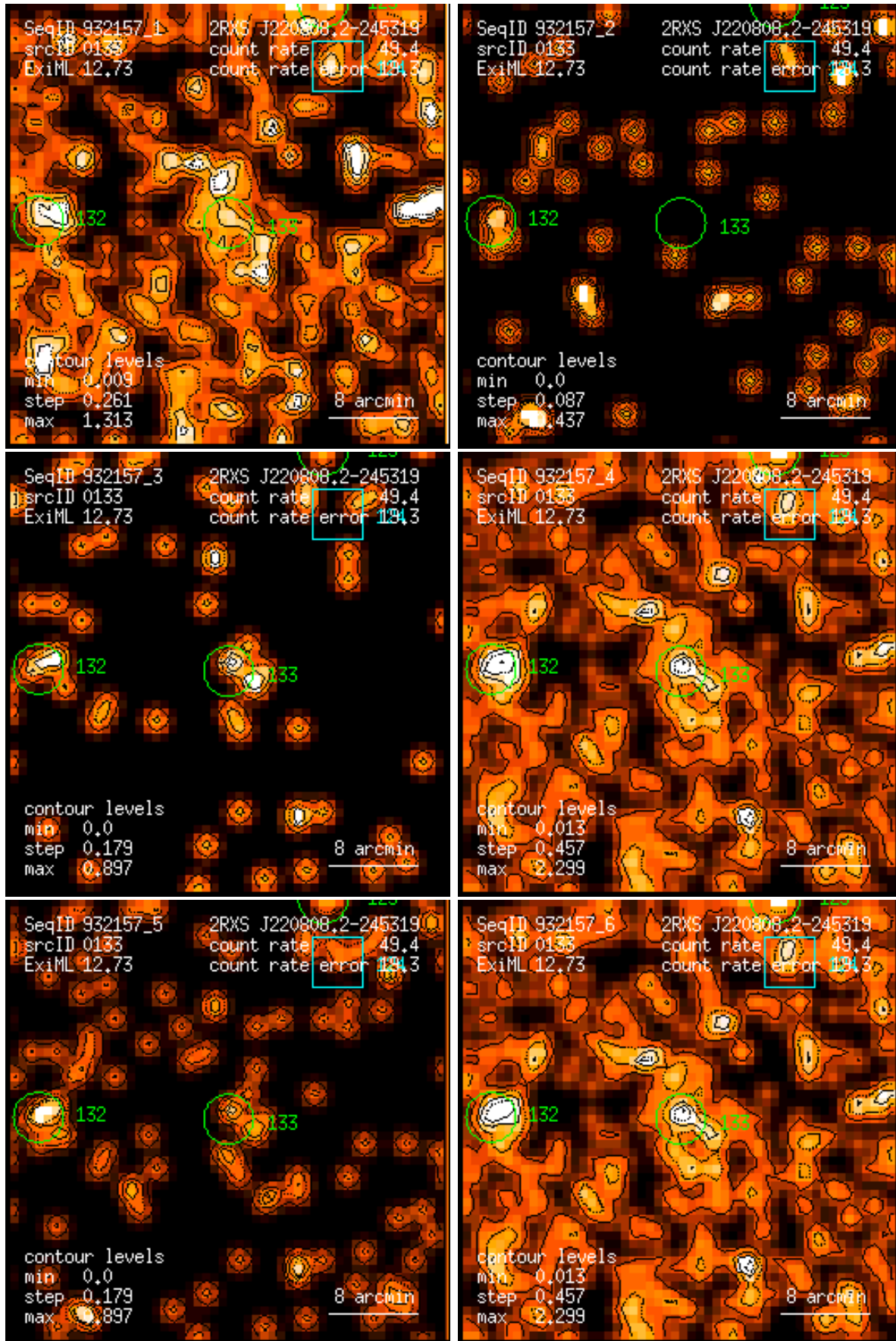
Figure 133: RASS 932157: detection 0133: band rate images, Gaussian filter: (1) PSPC channels 11 – 41, (2) 52 – 90, (3) 91 – 201, (4) 11 – 235, (5) 52 – 201, (6) 11 – 201. Broad band rates in counts/ks. Band rate contour levels in counts/ks/arcmin 2 .
