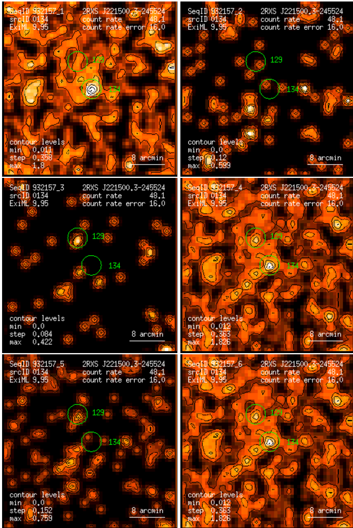
Figure 134: RASS 932157: detection 0134: band rate images, Gaussian filter: (1) PSPC channels 11 – 41, (2) 52 – 90, (3) 91 – 201, (4) 11 – 235, (5) 52 – 201, (6) 11 – 201. Broad band rates in counts/ks. Band rate contour levels in counts/ks/arcmin 2 .
