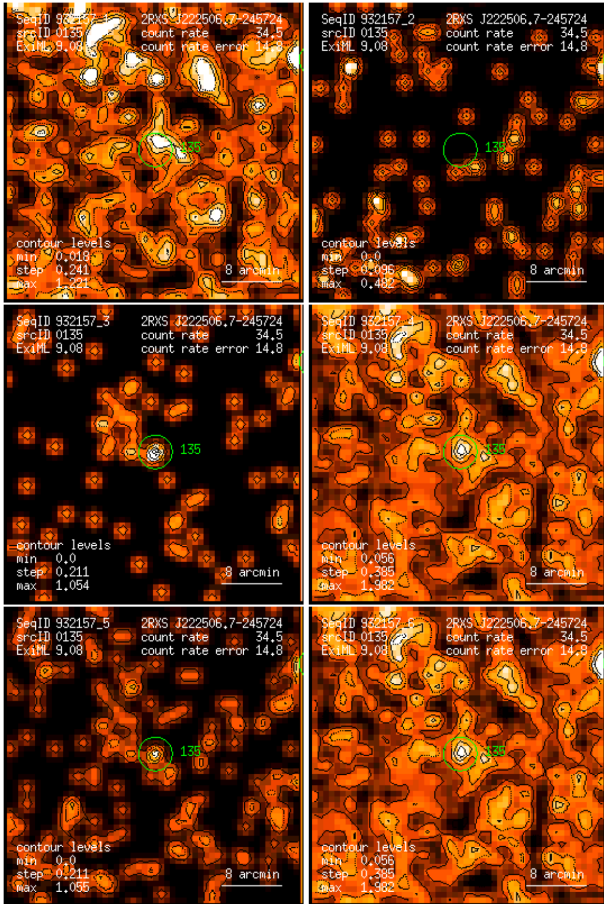
Figure 135: RASS 932157: detection 0135: band rate images, Gaussian filter: (1) PSPC channels 11 – 41, (2) 52 – 90, (3) 91 – 201, (4) 11 – 235, (5) 52 – 201, (6) 11 – 201. Broad band rates in counts/ks. Band rate contour levels in counts/ks/arcmin 2 .
