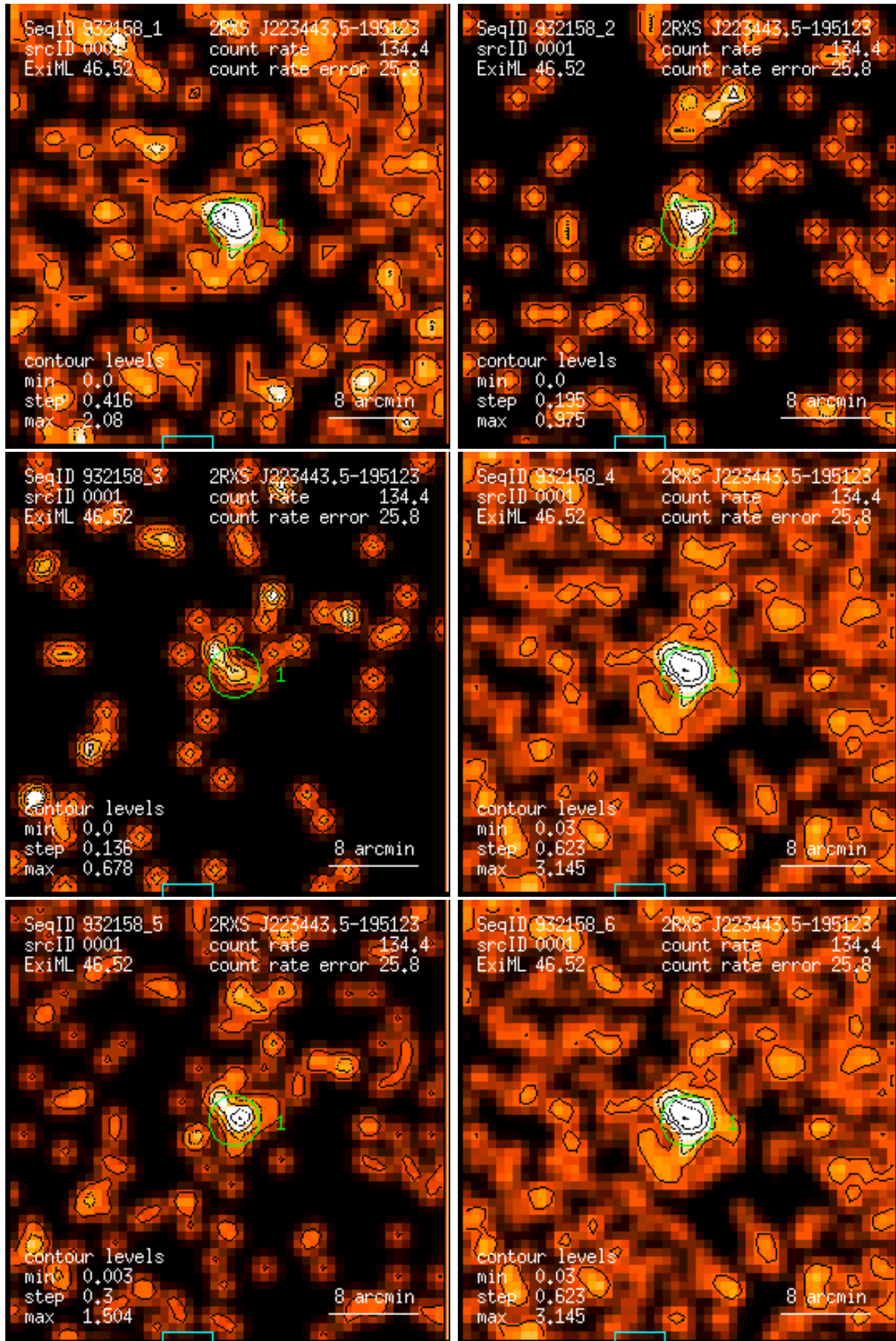
Figure 1: RASS 932158: detection 0001: band rate images, Gaussian filter: (1) PSPC channels 11 – 41, (2) 52 – 90, (3) 91 – 201, (4) 11 – 235, (5) 52 – 201, (6) 11 – 201. Broad band rates in counts/ks. Band rate contour levels in counts/ks/arcmin 2 .
