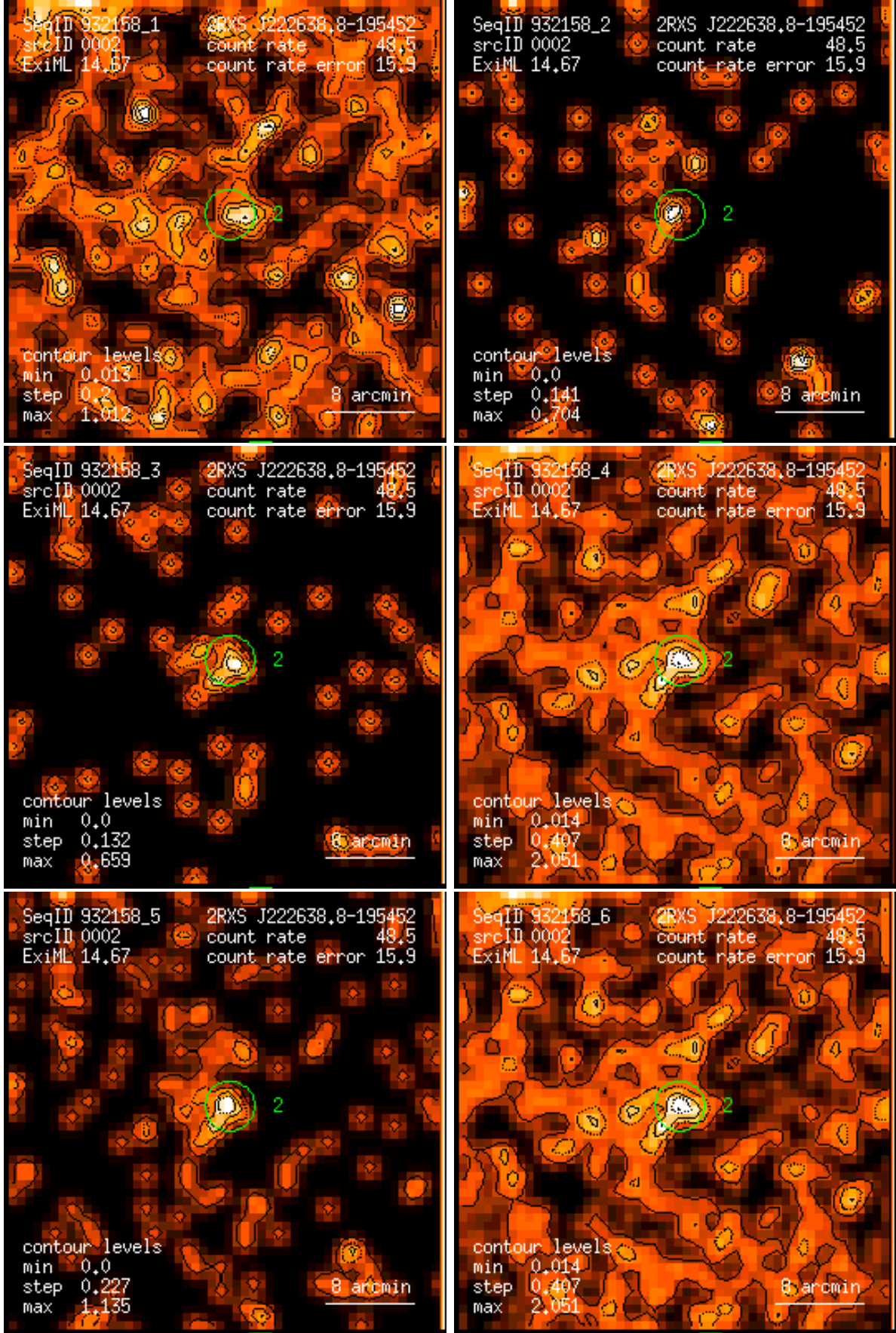
Figure 2: RASS 932158: detection 0002: band rate images, Gaussian filter: (1) PSPC channels 11 – 41, (2) 52 – 90, (3) 91 – 201, (4) 11 – 235, (5) 52 – 201, (6) 11 – 201. Broad band rates in counts/ks. Band rate contour levels in counts/ks/arcmin 2 .
