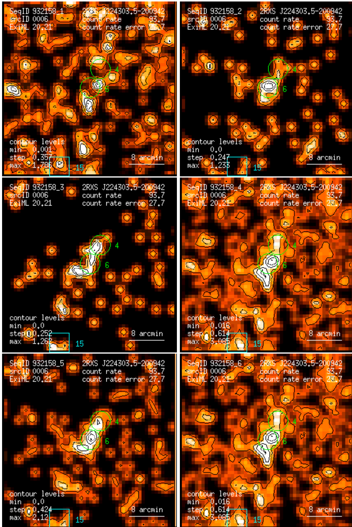
Figure 6: RASS 932158: detection 0006: band rate images, Gaussian filter: (1) PSPC channels 11 – 41, (2) 52 – 90, (3) 91 – 201, (4) 11 – 235, (5) 52 – 201, (6) 11 – 201. Broad band rates in counts/ks. Band rate contour levels in counts/ks/arcmin 2 .
