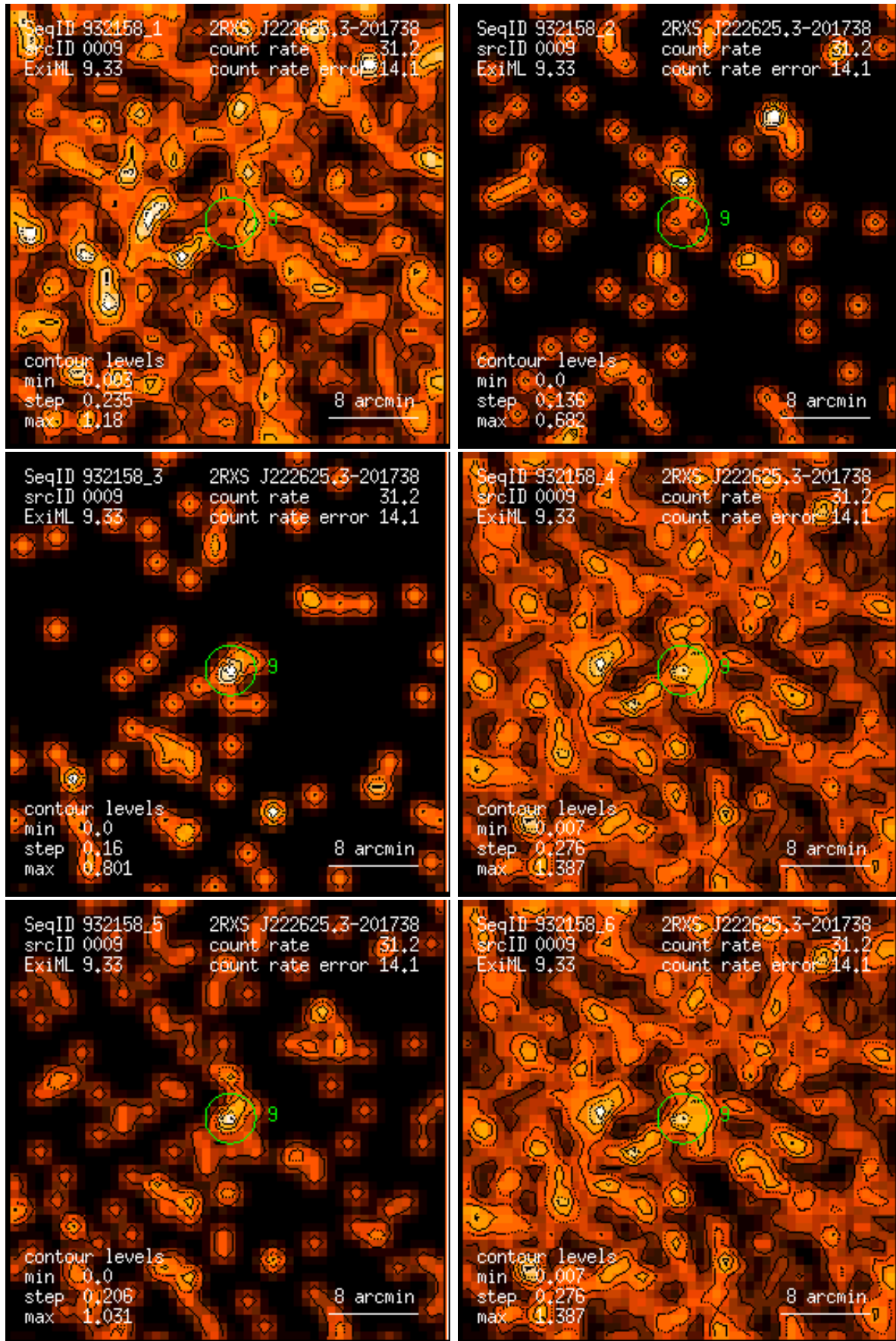
Figure 9: RASS 932158: detection 0009: band rate images, Gaussian filter: (1) PSPC channels 11 – 41, (2) 52 – 90, (3) 91 – 201, (4) 11 – 235, (5) 52 – 201, (6) 11 – 201. Broad band rates in counts/ks. Band rate contour levels in counts/ks/arcmin 2 .
