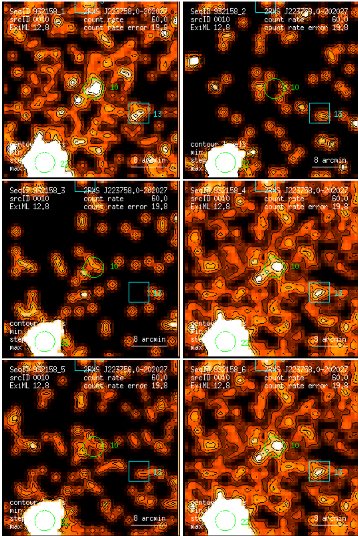
Figure 10: RASS 932158: detection 0010: band rate images, Gaussian filter: (1) PSPC channels 11 – 41, (2) 52 – 90, (3) 91 – 201, (4) 11 – 235, (5) 52 – 201, (6) 11 – 201. Broad band rates in counts/ks. Band rate contour levels in counts/ks/arcmin 2 .
