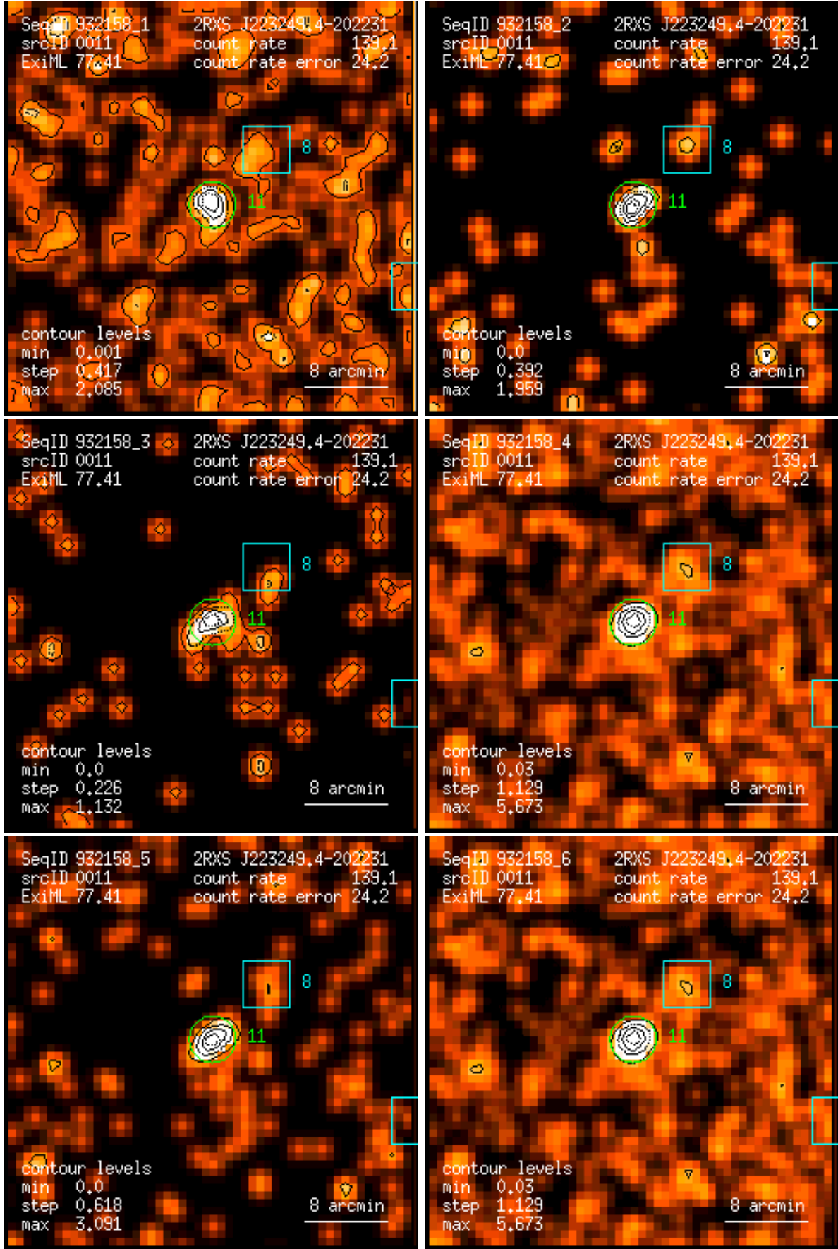
Figure 11: RASS 932158: detection 0011: band rate images, Gaussian filter: (1) PSPC channels 11 – 41, (2) 52 – 90, (3) 91 – 201, (4) 11 – 235, (5) 52 – 201, (6) 11 – 201. Broad band rates in counts/ks. Band rate contour levels in counts/ks/arcmin 2 .
