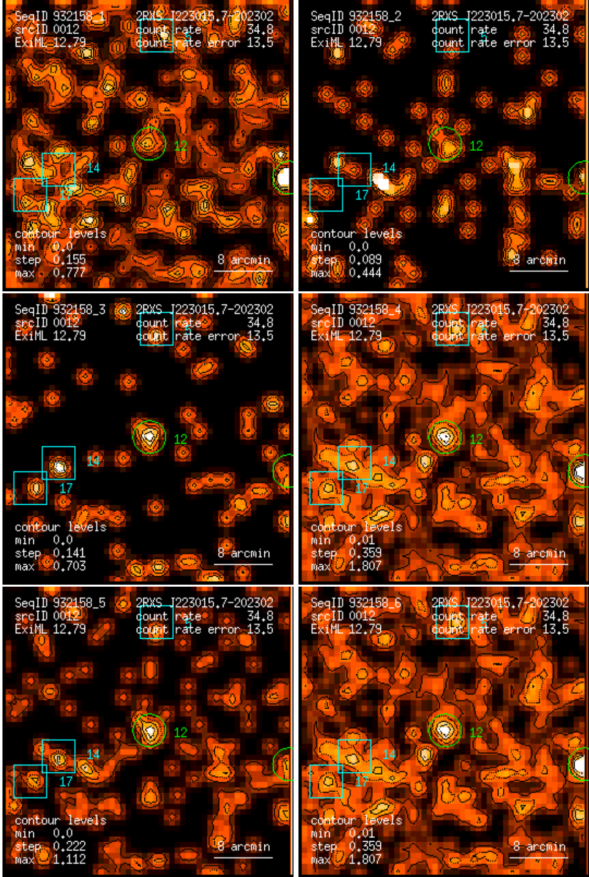
Figure 12: RASS 932158: detection 0012: band rate images, Gaussian filter: (1) PSPC channels 11 – 41, (2) 52 – 90, (3) 91 – 201, (4) 11 – 235, (5) 52 – 201, (6) 11 – 201. Broad band rates in counts/ks. Band rate contour levels in counts/ks/arcmin 2 .
