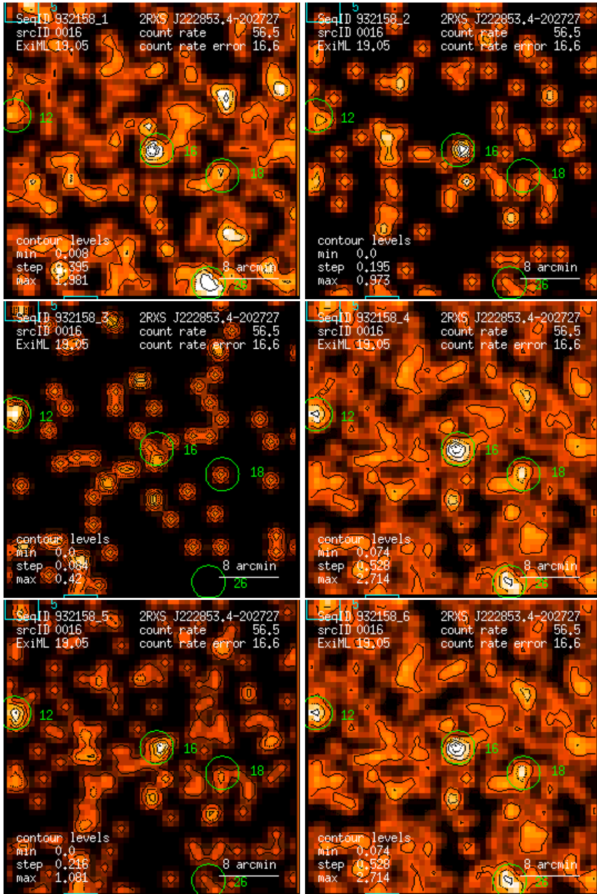
Figure 16: RASS 932158: detection 0016: band rate images, Gaussian filter: (1) PSPC channels 11 – 41, (2) 52 – 90, (3) 91 – 201, (4) 11 – 235, (5) 52 – 201, (6) 11 – 201. Broad band rates in counts/ks. Band rate contour levels in counts/ks/arcmin 2 .
