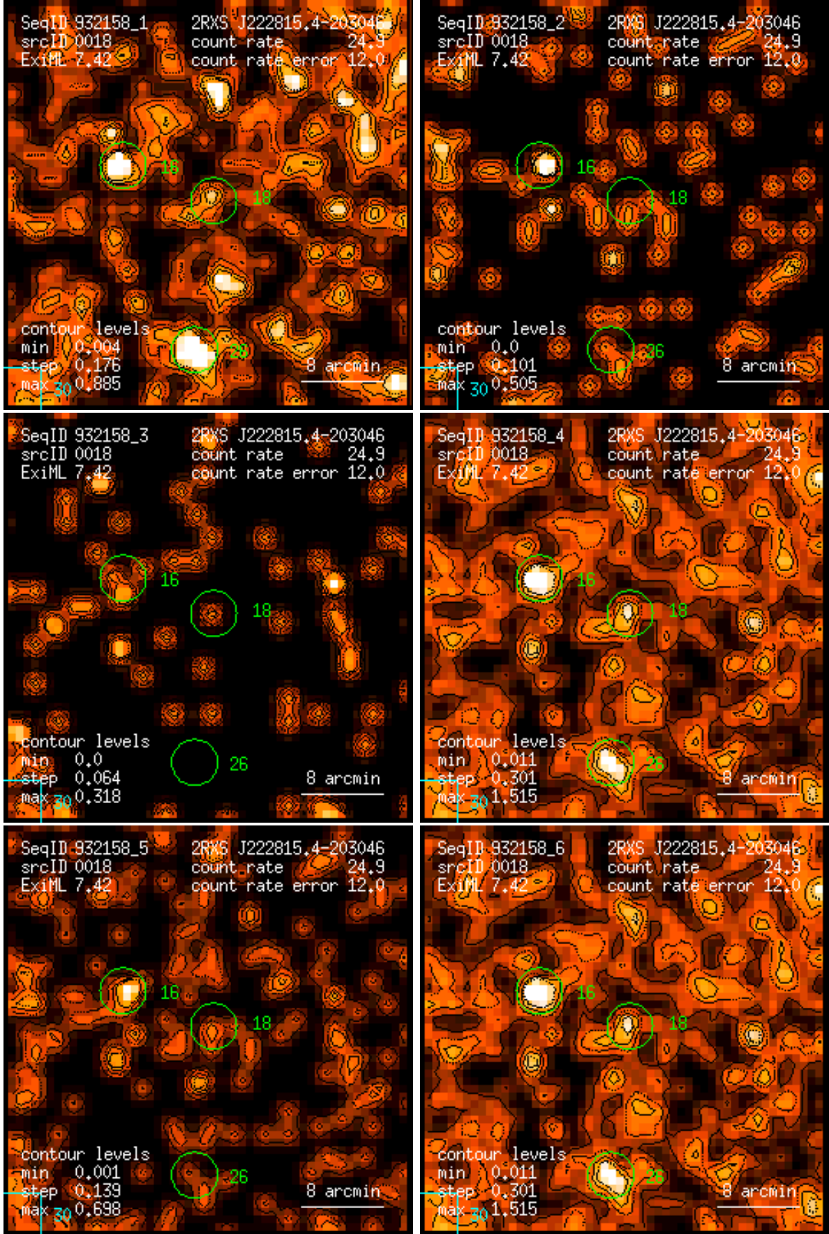
Figure 18: RASS 932158: detection 0018: band rate images, Gaussian filter: (1) PSPC channels 11 – 41, (2) 52 – 90, (3) 91 – 201, (4) 11 – 235, (5) 52 – 201, (6) 11 – 201. Broad band rates in counts/ks. Band rate contour levels in counts/ks/arcmin 2 .
