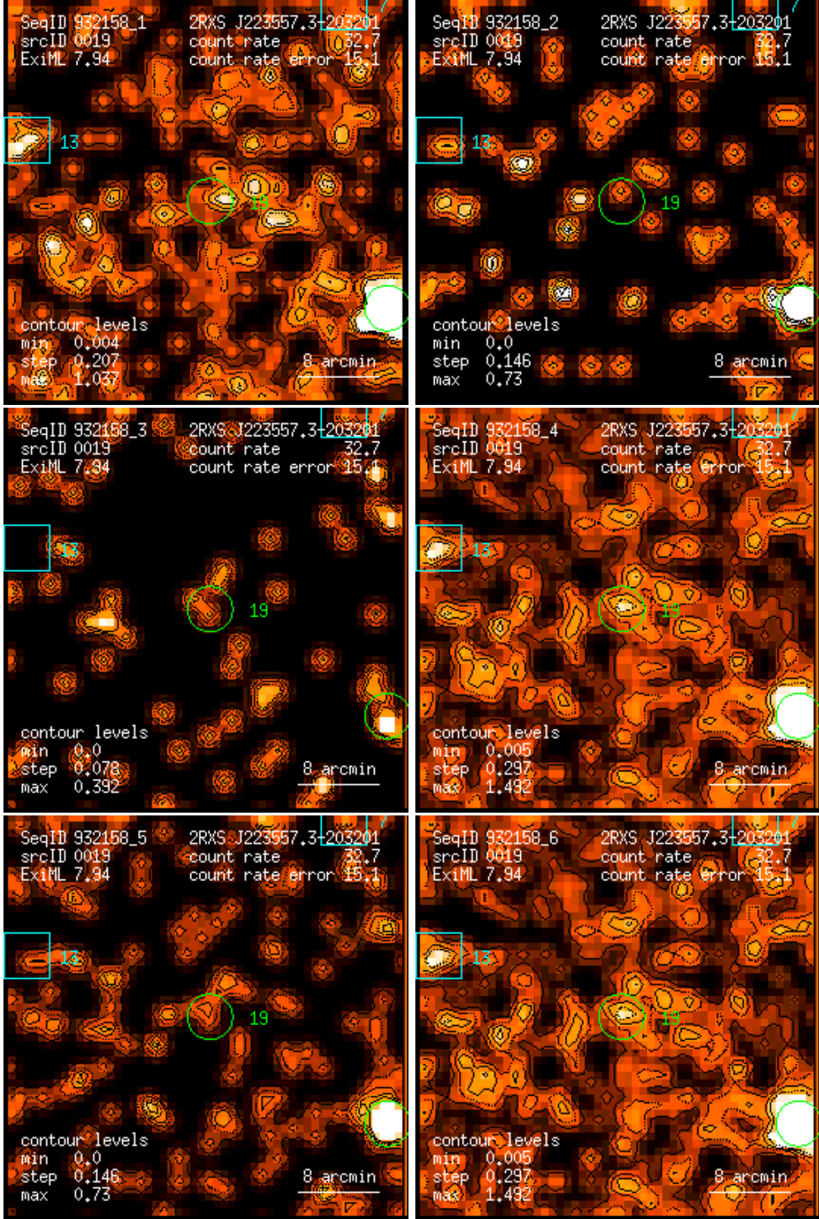
Figure 19: RASS 932158: detection 0019: band rate images, Gaussian filter: (1) PSPC channels 11 – 41, (2) 52 – 90, (3) 91 – 201, (4) 11 – 235, (5) 52 – 201, (6) 11 – 201. Broad band rates in counts/ks. Band rate contour levels in counts/ks/arcmin 2 .
